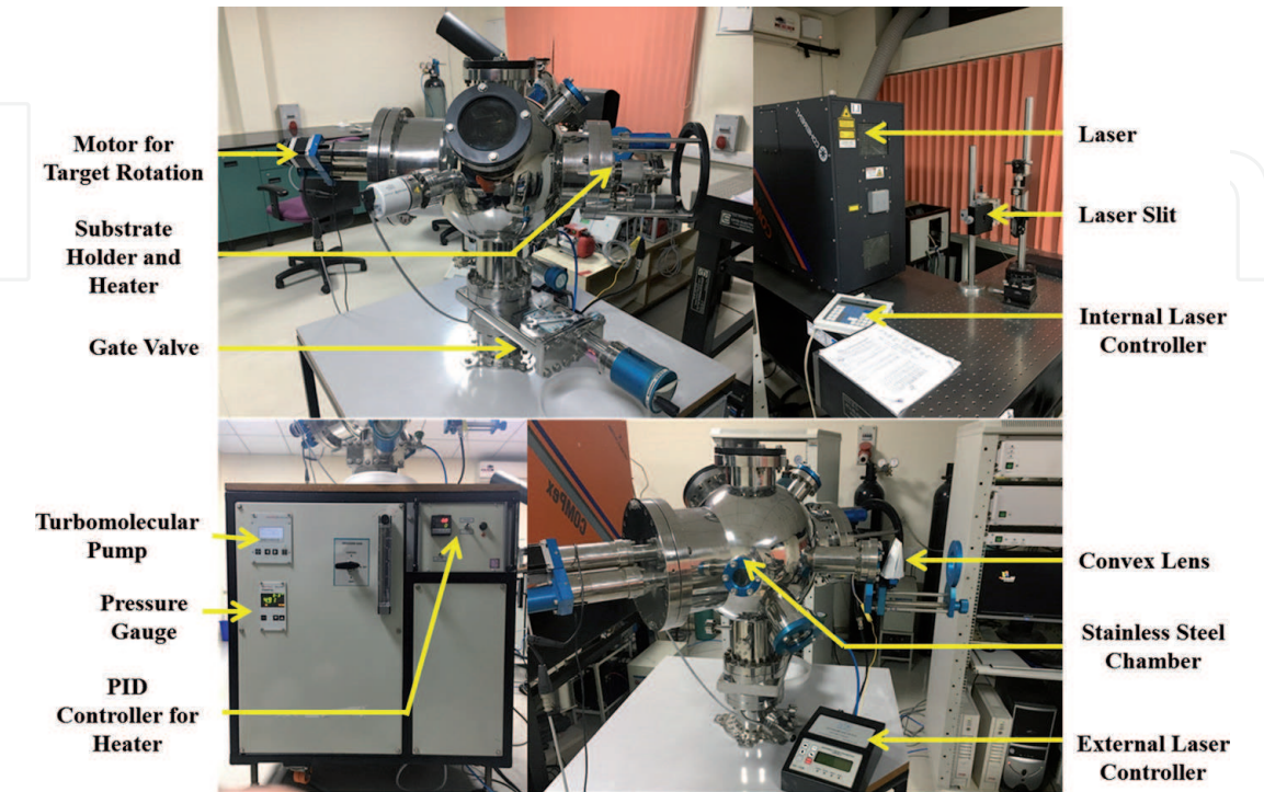
Figure 3. PLD setup in Materials Research Centre, Indian Institute of Science, Bangalore, India.
