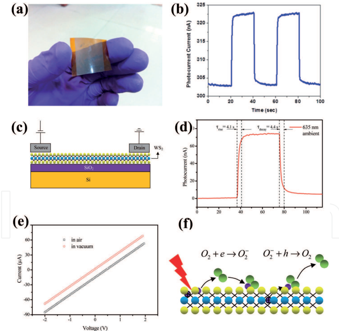
Figure 4. (a) MoS 2 thin film deposited on flexible kapton substrate and (b) temporal response of the device in zero-bias mode. Figures have been reproduced with permission from Ref. [60]. (c) Cross-sectional schematic view of the WS 2 -based photoresistor, (d) temporal response of the device in air, (e) I-V curves of the WS 2 -based device in vacuum and in air, and (f) schematic of the photodetection mechanism based on adsorption and desorption of O 2 molecules. Figures have been reproduced with permission from Ref. [47].
