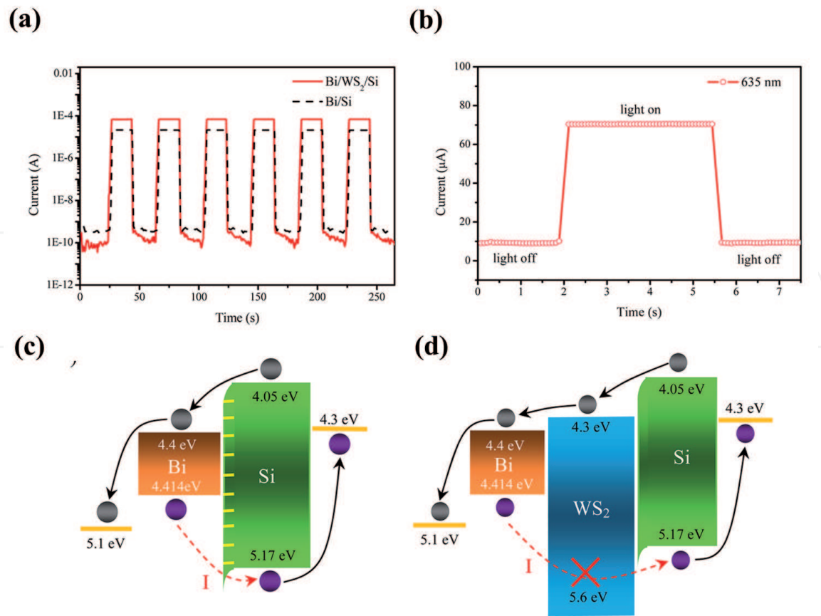
Figure 6. (a) Transient behavior of the Bi/Si and Bi/WS 2 /Si PDs under zero bias. (b) Corresponding single on-off cycle. Schematic of the energy band diagrams of the (c) Bi/Si and (d) Bi/WS 2 /Si heterointerfaces. Figures have been reproduced with permission from Ref. [75].
