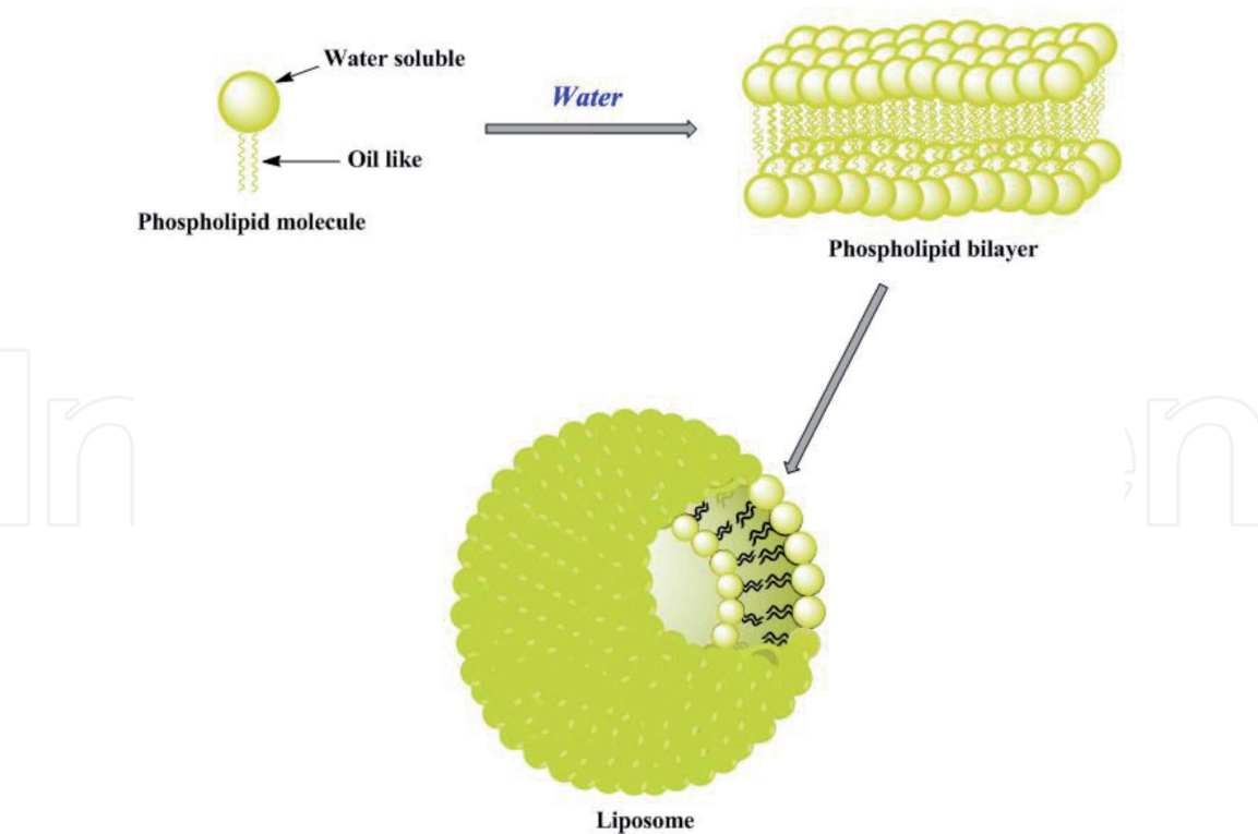
Figure 5. Mechanism of liposome formation.
