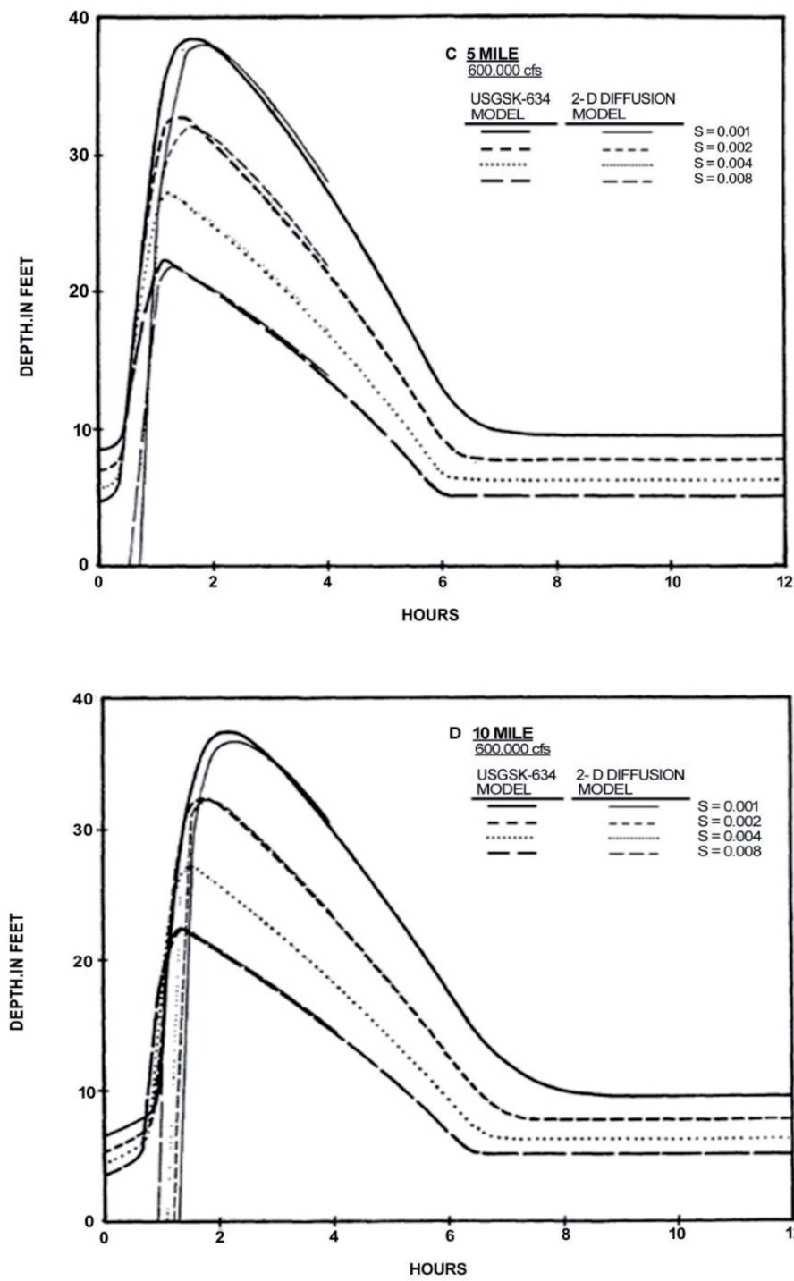
Figure 5. Comparisons of depths of water at 5 and 10 miles downstream from the dam-break site (peak Q = 600,000 cfs).
