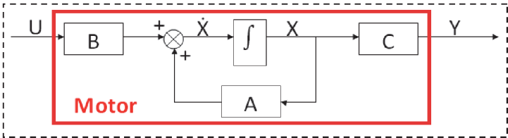
Figure 2. Induction motor state space mathematical model.
