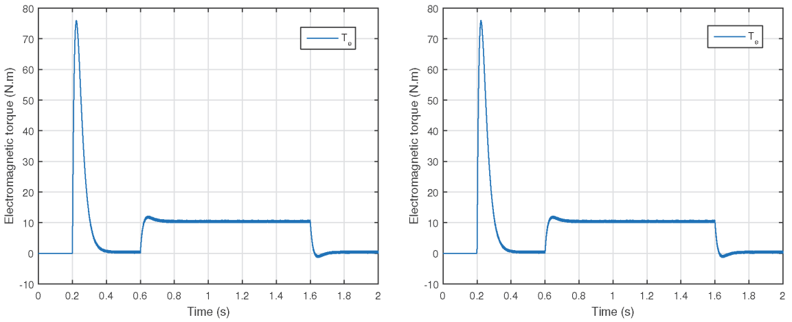
Figure 8. Electromagnetic torque response.
