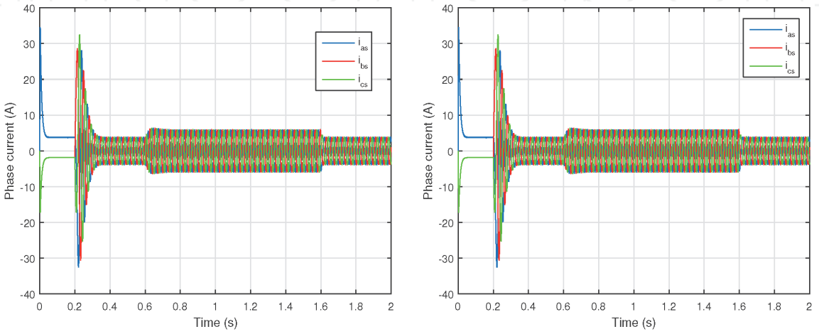
Figure 9. Stator phase currents response.
