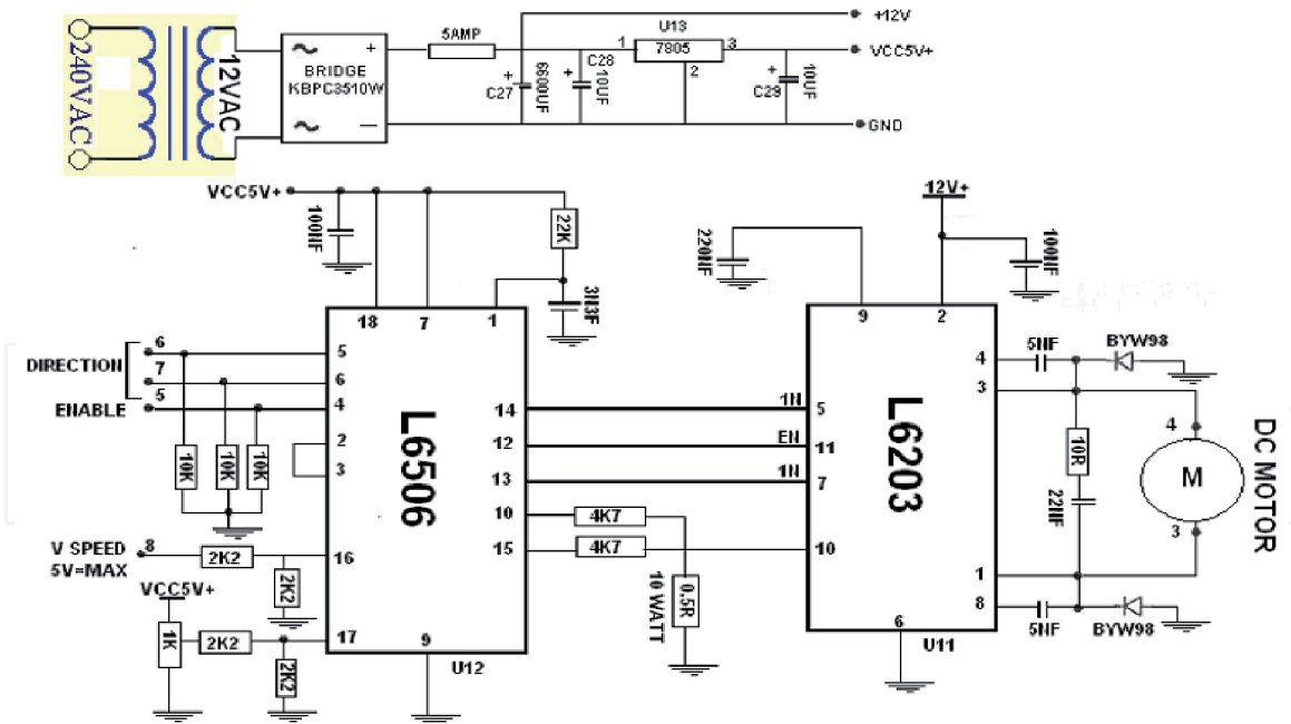
Figure 3. Schematic diagram for speed and direction control module for two dc motor.
