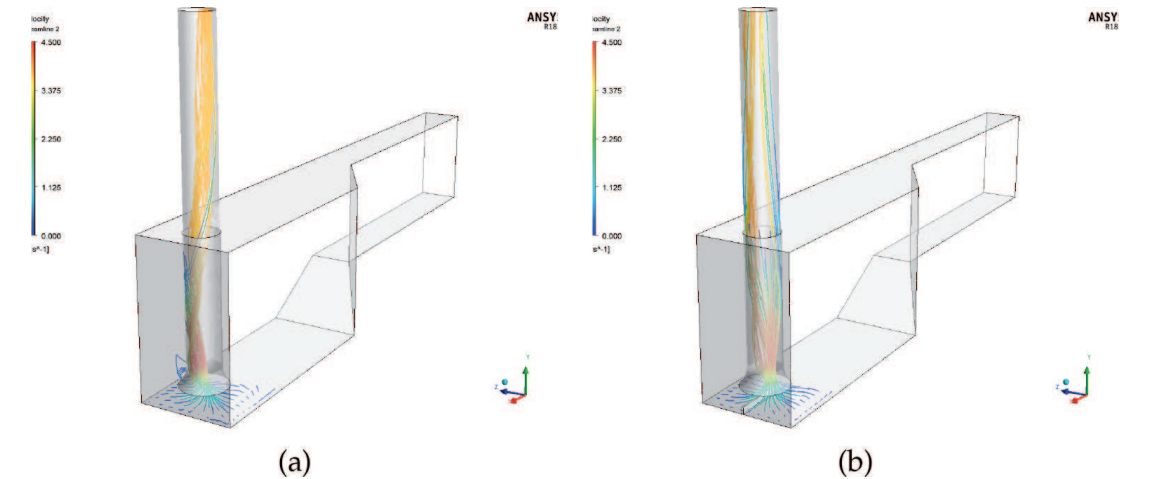
Figure 18. 3D streamline plot showing the intake flow in the sump with the seeding of the flow starts at the floor of the sump; (a) without floor splitter plate, (b) with floor splitter plate.
