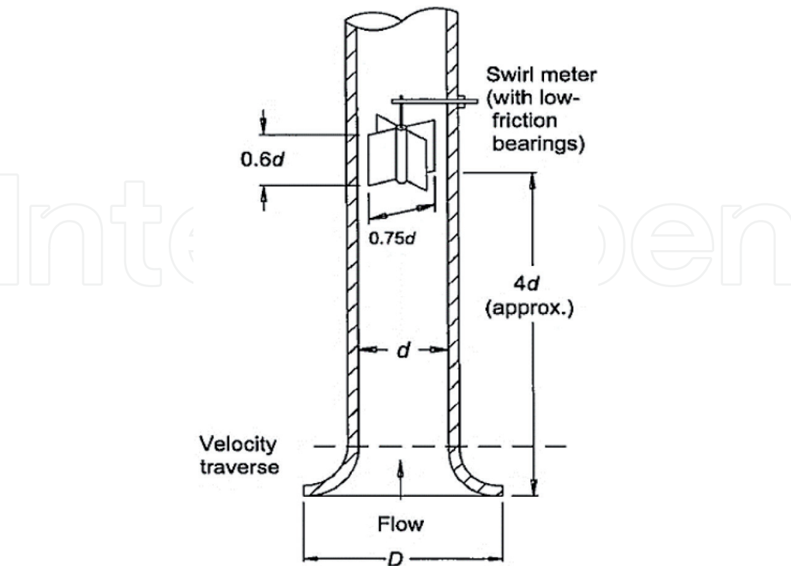
Figure 3. Swirl metre installation according to ANSI/HI 9.8-2018 standard.
