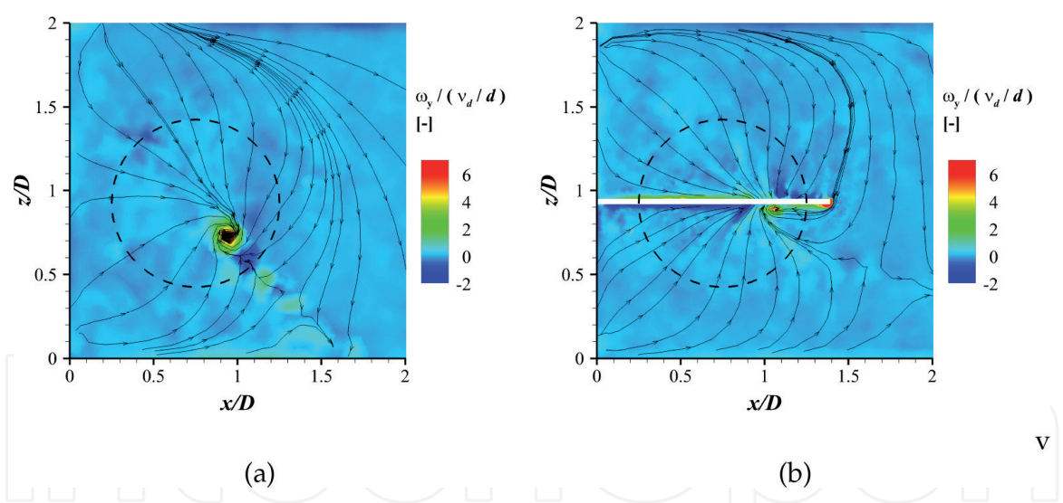
Figure 14. Contour plot of \omega_y / (v_d / d) at the floor of the sump in z-x plane; (a) without floor splitter plate, (b) with floor splitter plate.
