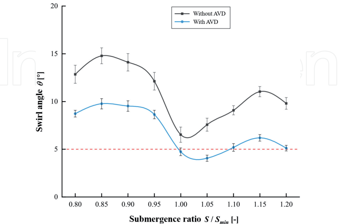
Figure 8. Swirl angle values at different submergence ratios for the false wall case.
