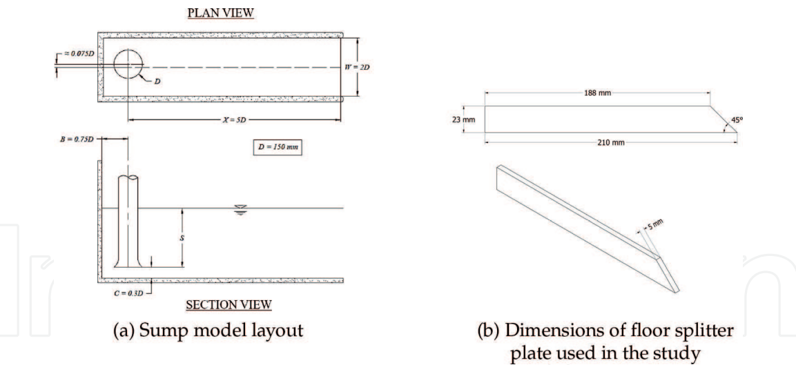
Figure 2. Main dimensions of the sump model and splitter.
