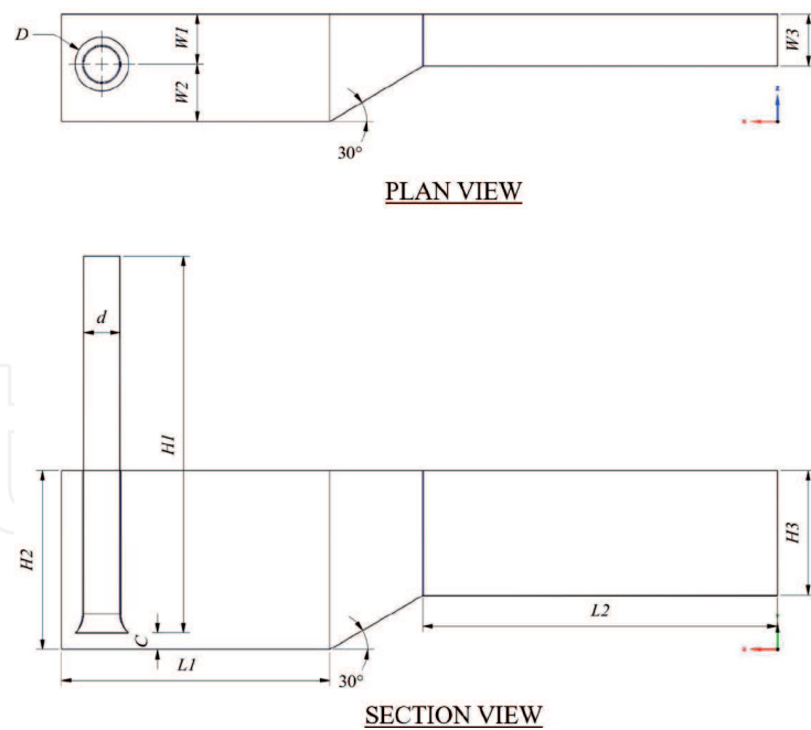
Figure 6. Dimensions of the full-scale model.
