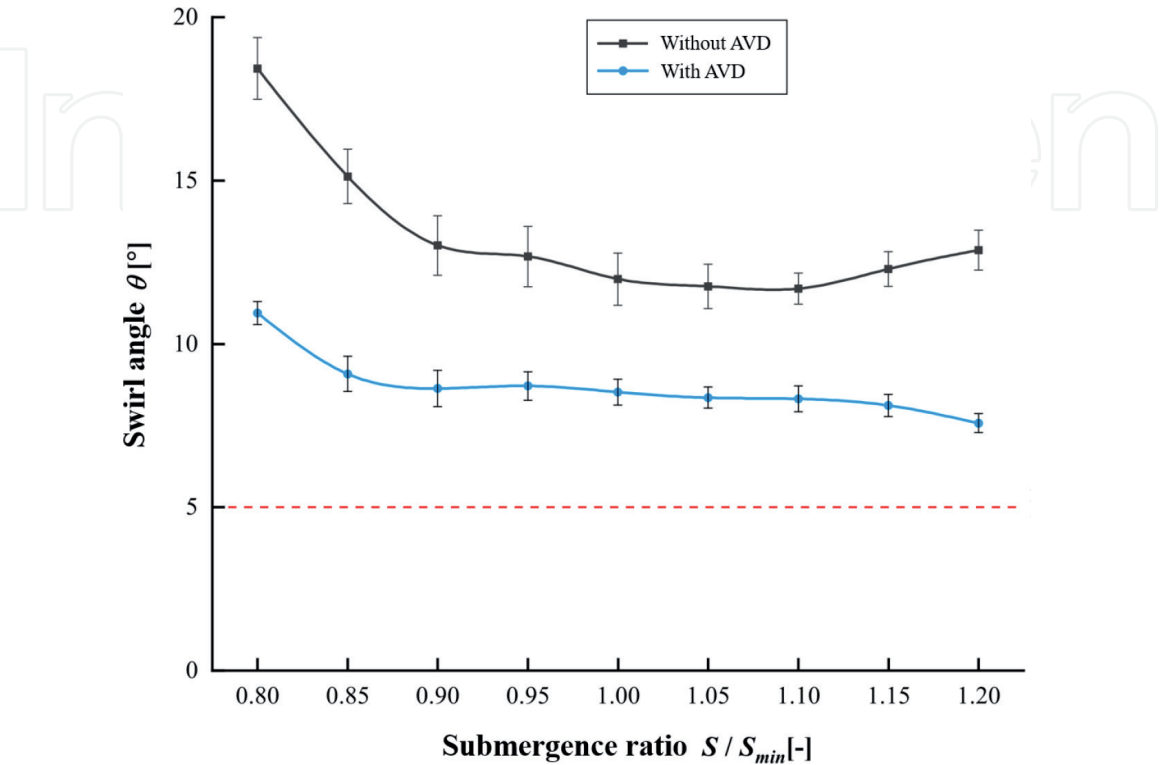
Figure 7. Swirl angle values at different submergence ratios for the false floor case.
