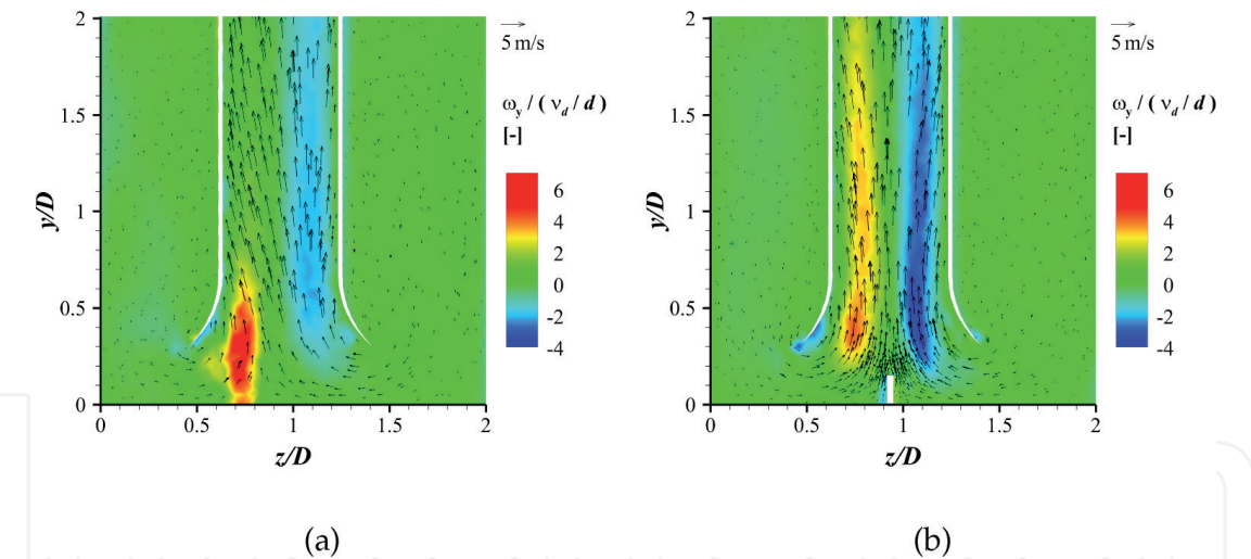
Figure 12. Contour plot of \omega_y / (v_d / d) at the location of vortex in y - z plane; (a) without floor splitter plate, (b) with floor splitter plate.
