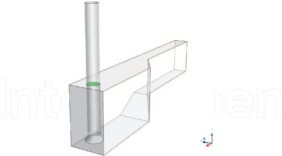
Figure 15. Evaluation area at the position of swirl metre in z-x plane of the pump sump model ( y = 4250\text{ mm} ).
