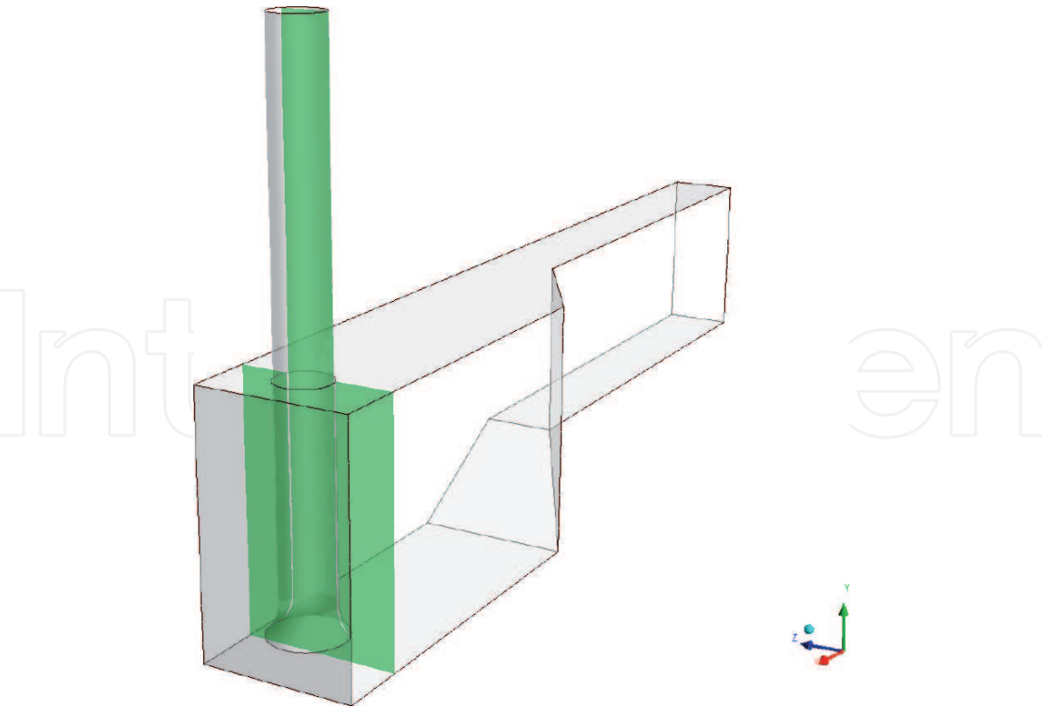
Figure 11. Evaluation area in y - z plane of the pump sump model ( x = 15,860 mm).
