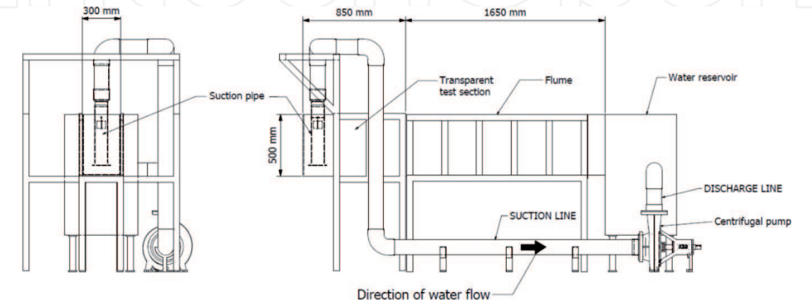
Figure 1. The experimental rig.
