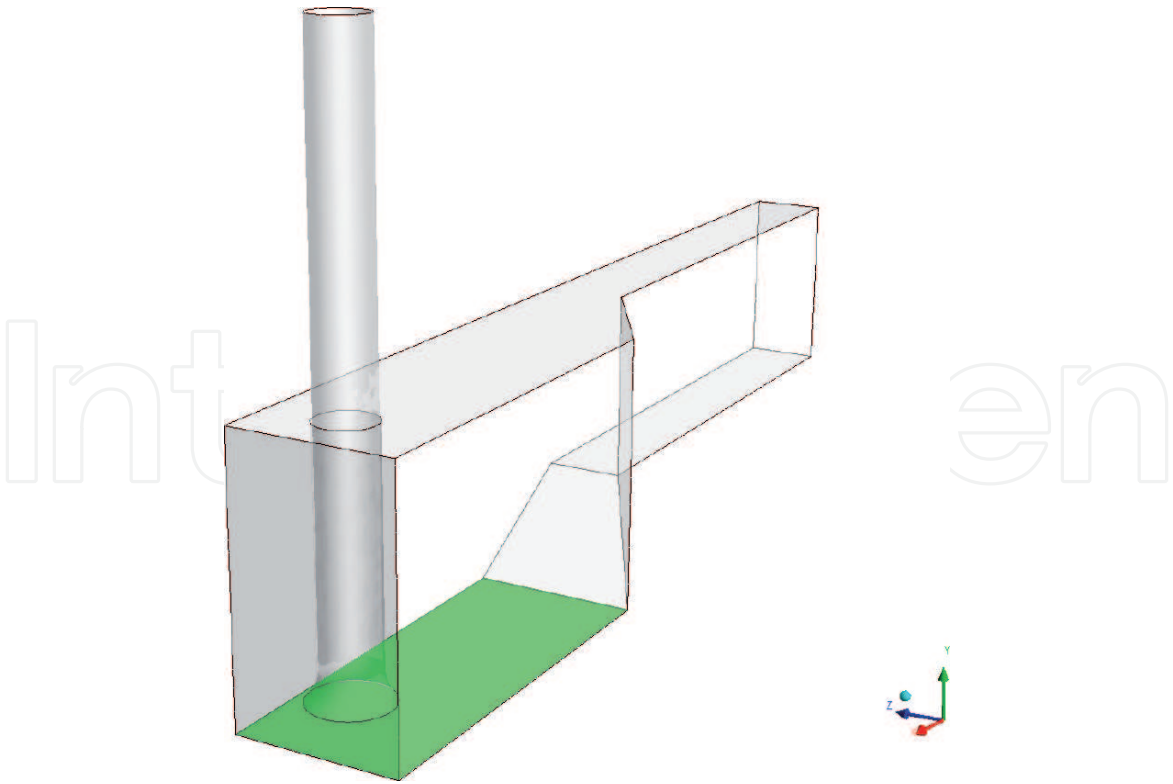
Figure 13. Evaluation area in z-x plane of the pump sump model ( y = 10\text{ mm} ).
