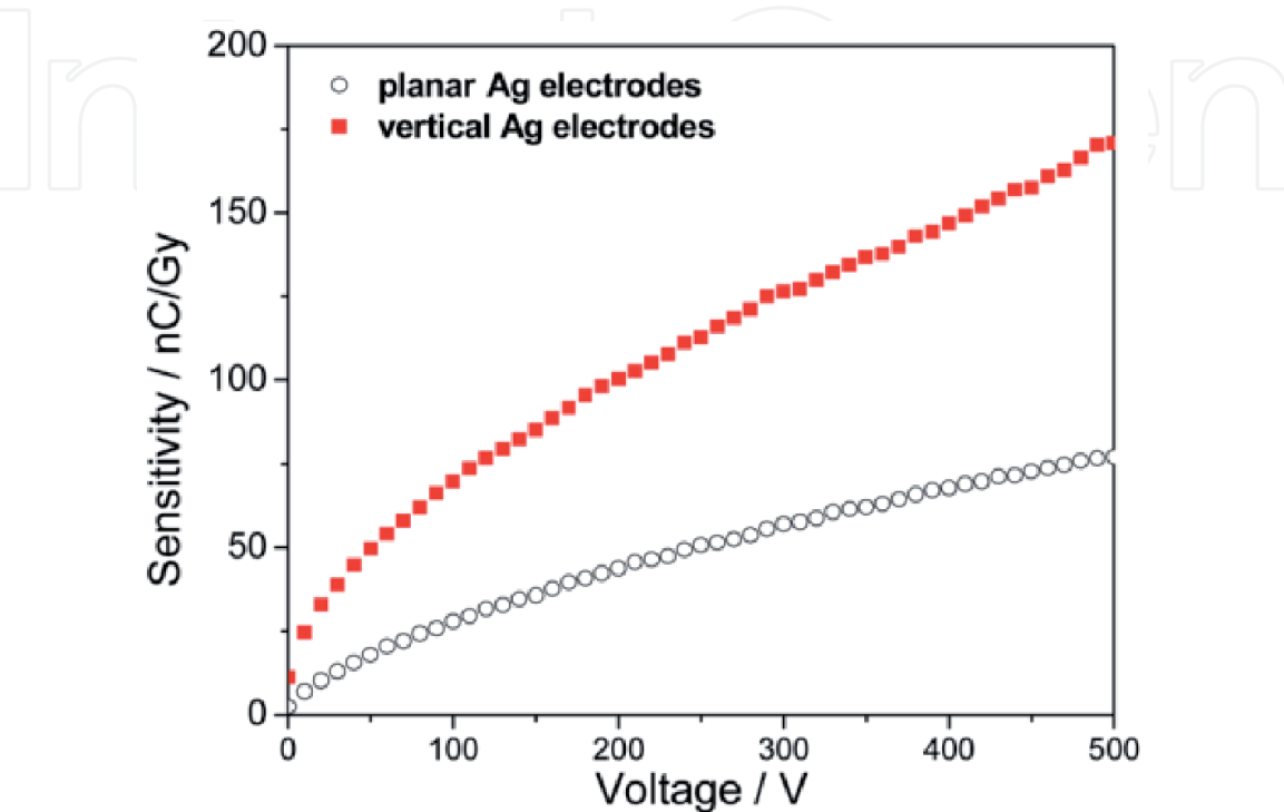
Figure 6. Comparison between the sensitivity values at different bias voltages for a 4HCB-based detector under 35 keV X-ray irradiation in the planar (black circles) and vertical (red squares) electrode configuration [26].
