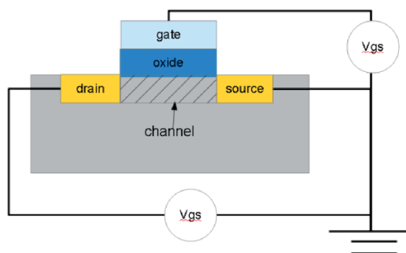
Figure 2. A metal oxide semiconductor field-effect transistor typical structure.
