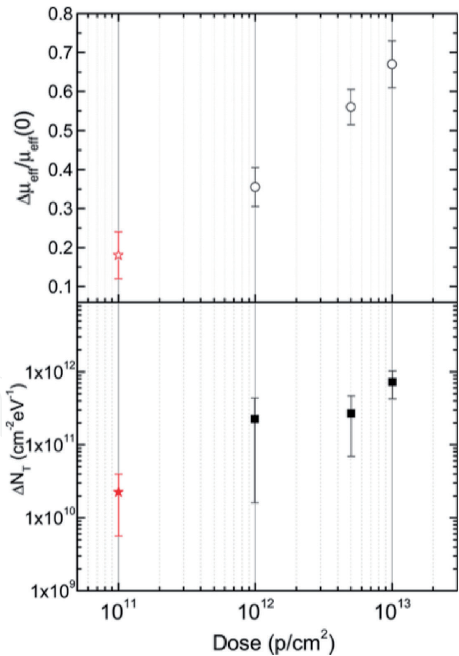
Figure 5. Variation of the trap densities, \Delta N_T (bottom solid squares), and of the channel mobility relative to \mu_{eff}(0) and \Delta\mu_{eff}/\mu_{eff}(0) (top open circles) as a function of the irradiation dose [20].
