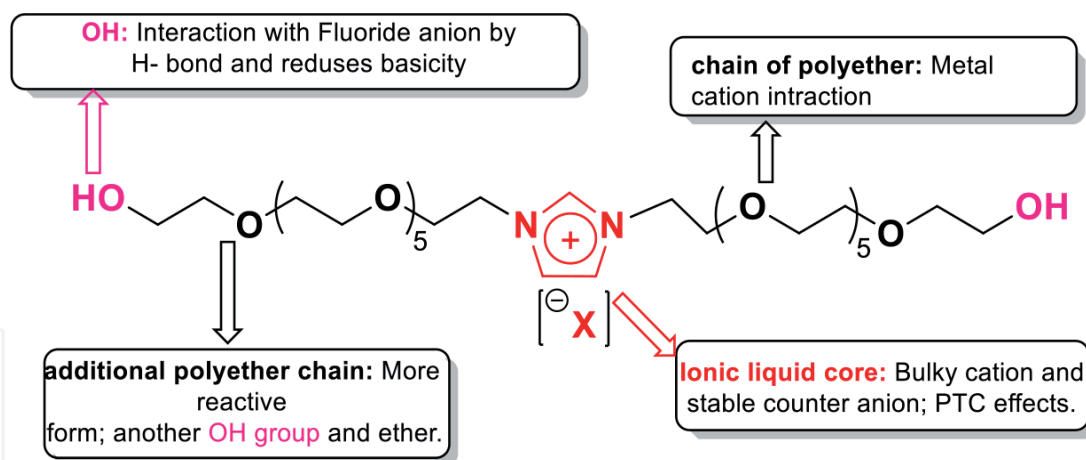
Figure 7. Di-functional polyether chain-substituted imidazolium IL.
