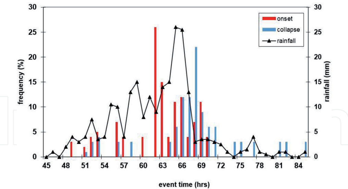
Figure 15. Relationship between precipitation and time of onset and collapse of translational block slides in the Langhe hills during the severe November 1994 event.
