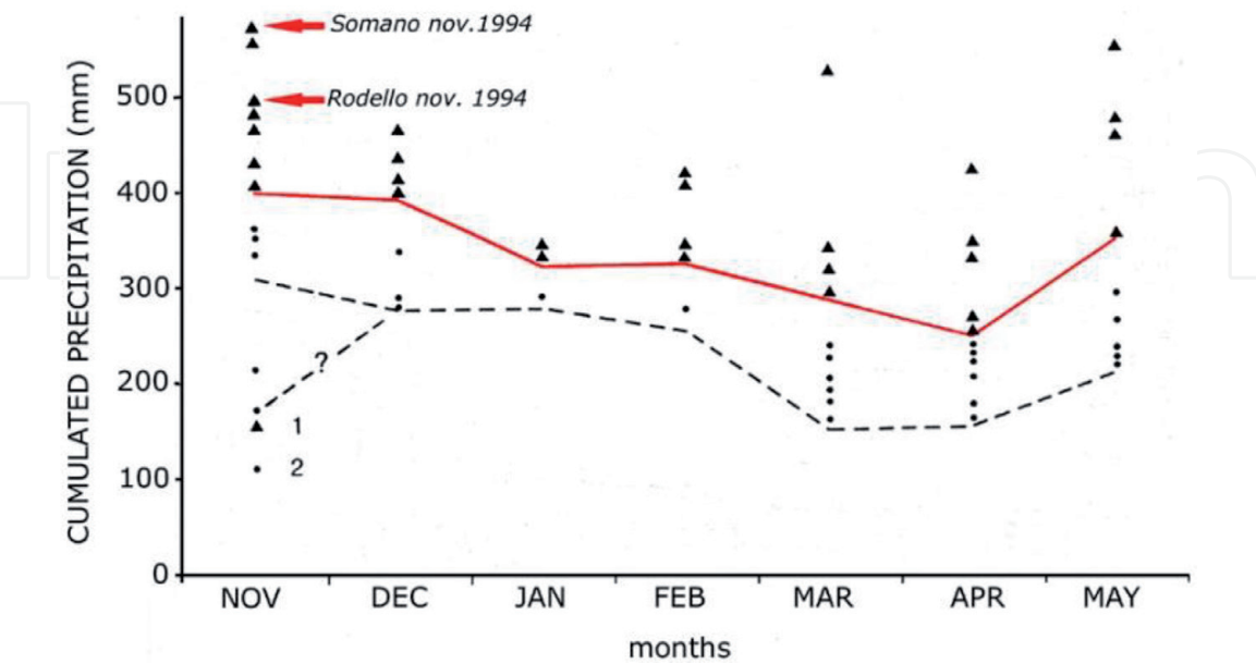
Figure 14. Diagram showing precipitation amounts triggering rock-block slides in the Langhe hills. The dashed line defines the area of minimum rainfall values in the 60 days before the collapse. The red line denotes the threshold total values (previous rainfall + event rainfall) that cause landslides (1 – cumulated precipitations triggering landslides; 2 – cumulated rainfalls that do not trigger landslides). The rainfall values triggering the Somano and Rodello TRBS occurred on November 1994 are indicated with a red arrow ([9], modified).
