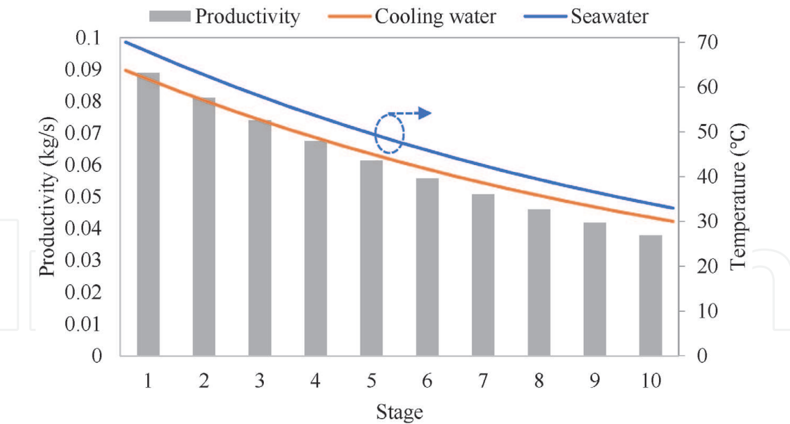
Figure 3. Temperature and production profile for a typical system with 10 production stages.
