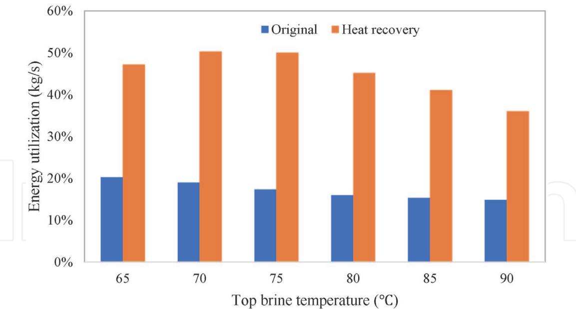
Figure 9. Comparison of energy utilization for the heat source before and after heat recovery.
