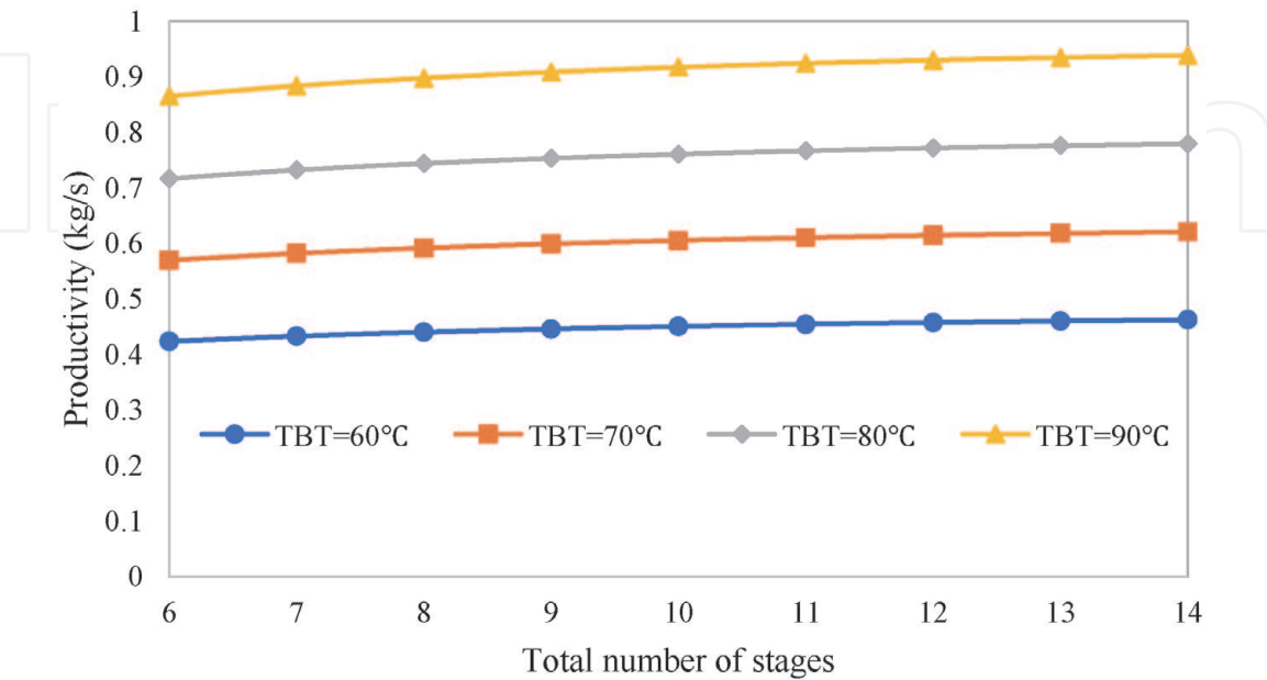
Figure 4. Productivity under different top brine temperatures and operating stages.
