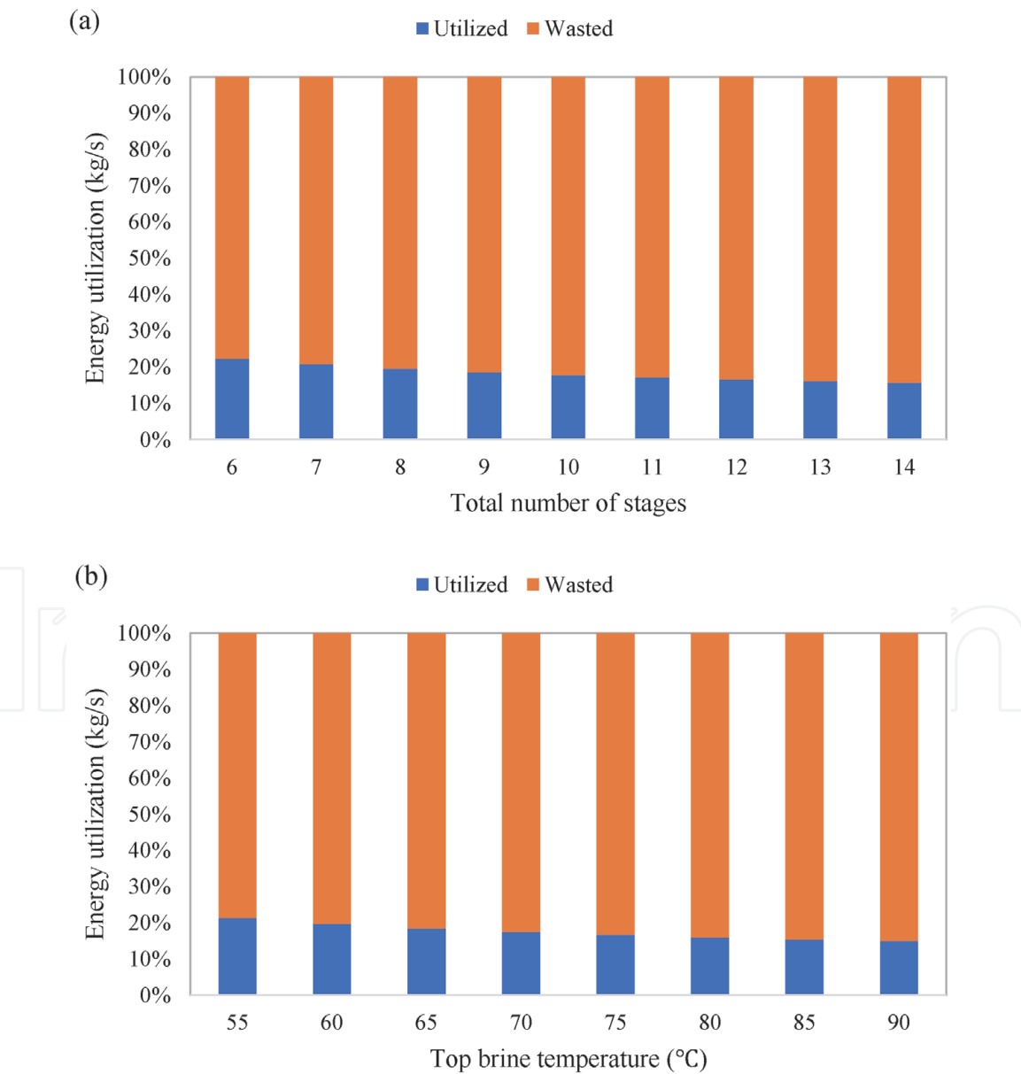
Figure 5. Level of energy utilization under different (a) numbers of operating stages and (b) top brine temperatures.
