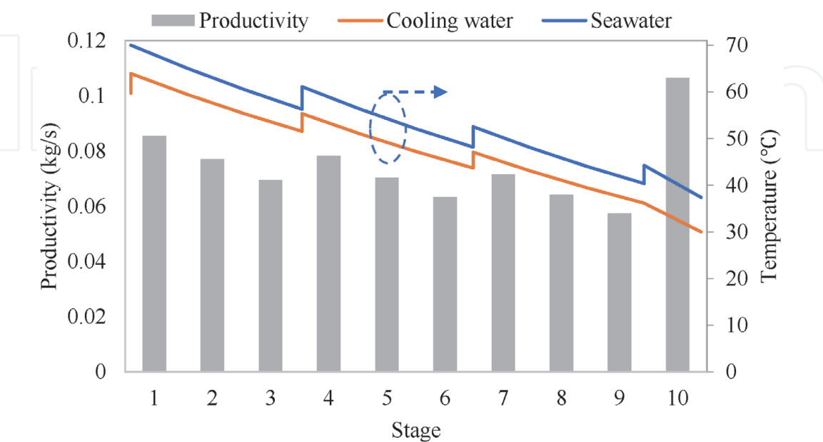
Figure 7. Temperature and productivity profile for the modified system.
