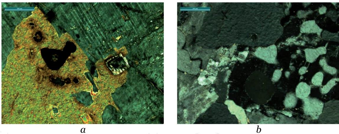
Figure 12. Thin skin of rapakivi granite: (a) plagioclase, microcline and biotite with pyrite and zircon; (b) quartz, plagioclase and microcline. XPL (a), PPL (b).
