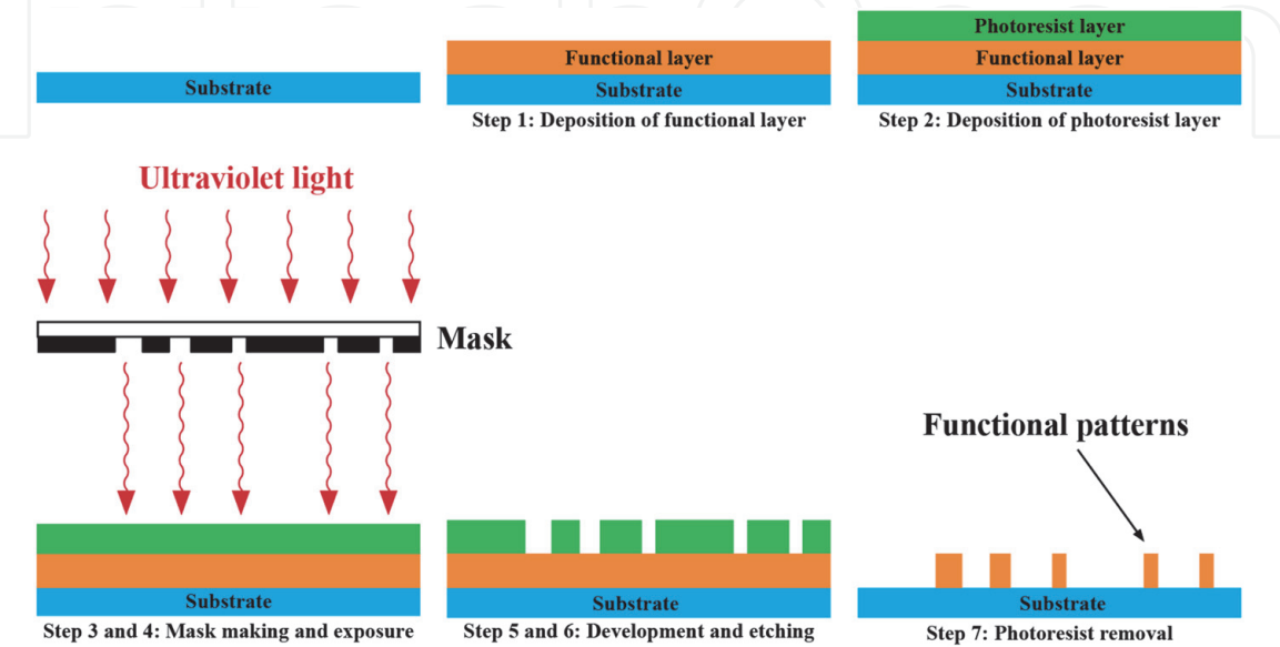
Figure 6. Subtractive manufacturing steps [16].
