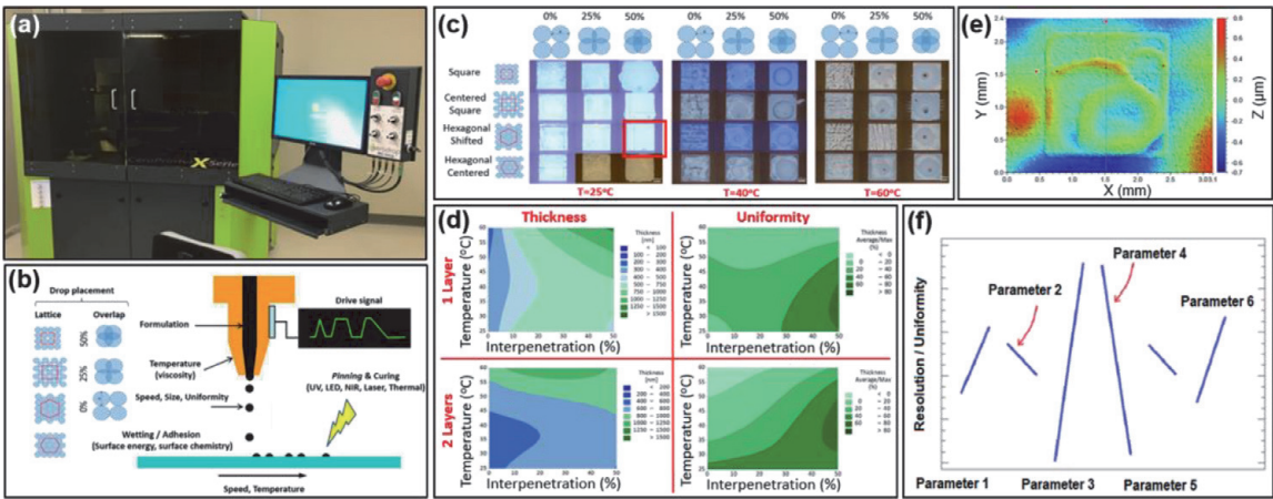
Figure 14. Digital inkjet printing process mapping and optimization. (a) Research grade Ceradrop digital inkjet printing system at ÉTS; (b) precise control of a wide range of critical jetting parameters; (c) examples of inkjet-printed features using Ag ink on Kapton® for different printing lattices (drop placement configurations), drop interpenetration, and substrate temperatures; (d) example of one-layer and two-layer process mappings looking at the Ag features' thickness and uniformity for different substrate temperatures and drop interpenetrations in the hexagonal shifted lattice configuration; (e) typical high-resolution laser-scanning microscope image of the features obtained using a hexagonal shifted lattice with 50% interpenetration at 25 °C substrate temperature; (f) example of a typical multivariate design-of-experiment analysis for process optimization (adapted from [94]).
