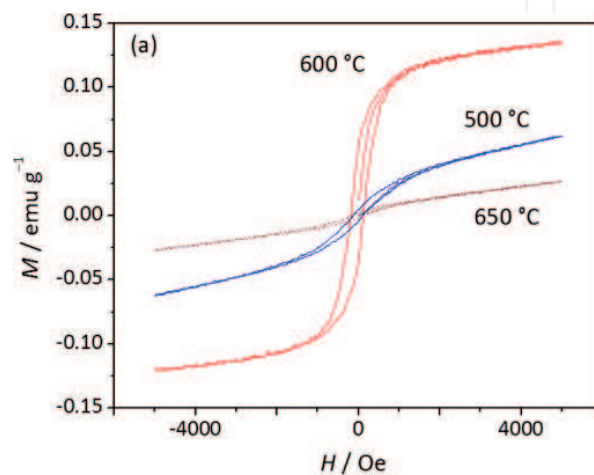
Figure 6. Fe doped SnO 2 magnetic hysteresis annealed for certain hours at different temperatures [54].
