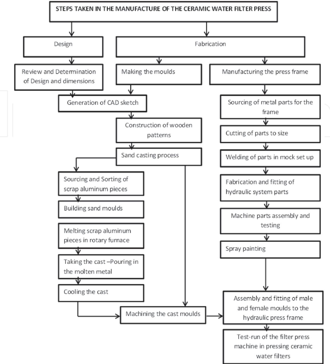
Flow chart of steps taken in fabricating the ceramic water filter press.
