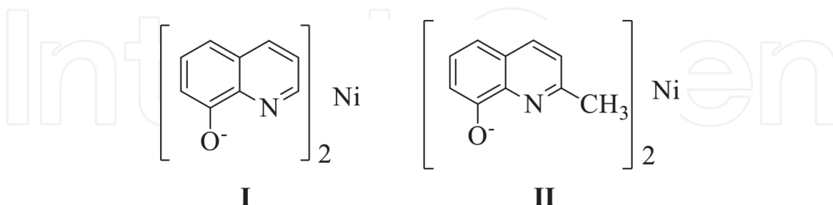
Figure 3. Chelating complexes of Ni(II) ion showing steric effect.
