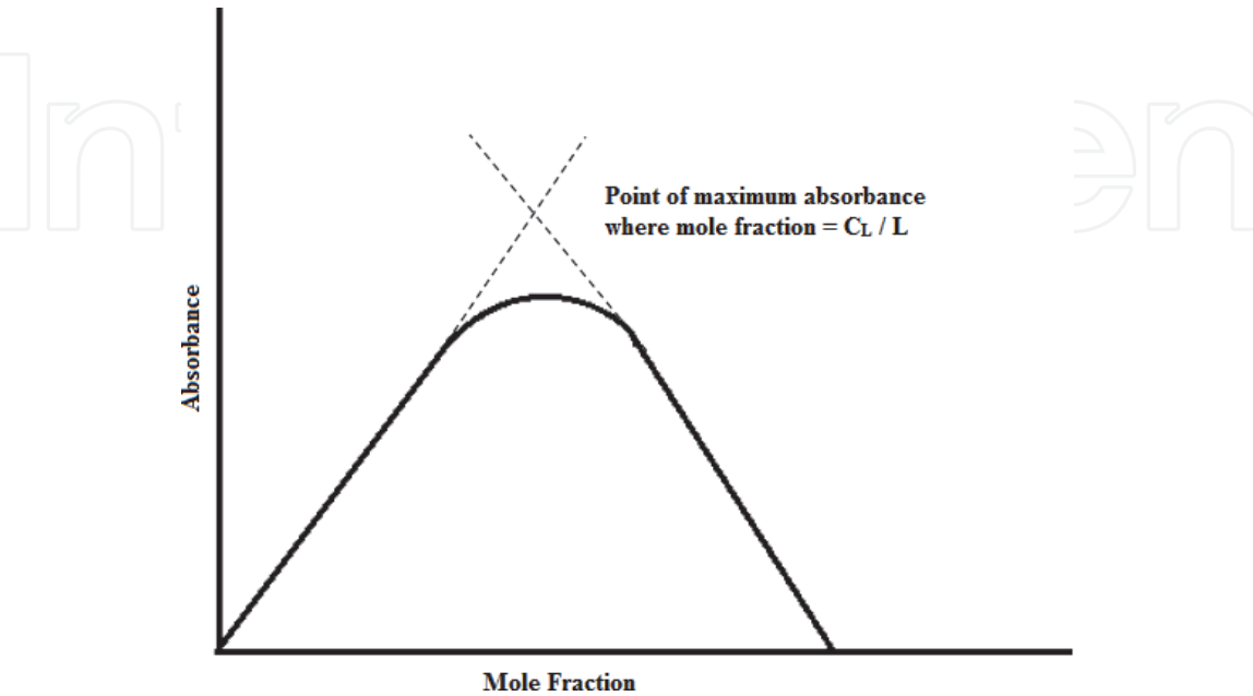
Figure 4. Determination of the composition of metal complex Job’s method of continuous variation.
