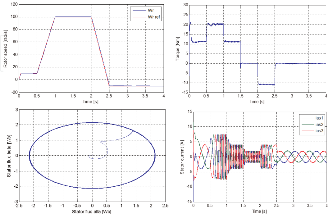
Figure 8. Simulation results of five-level DTC-ANN for low-speed operation.
