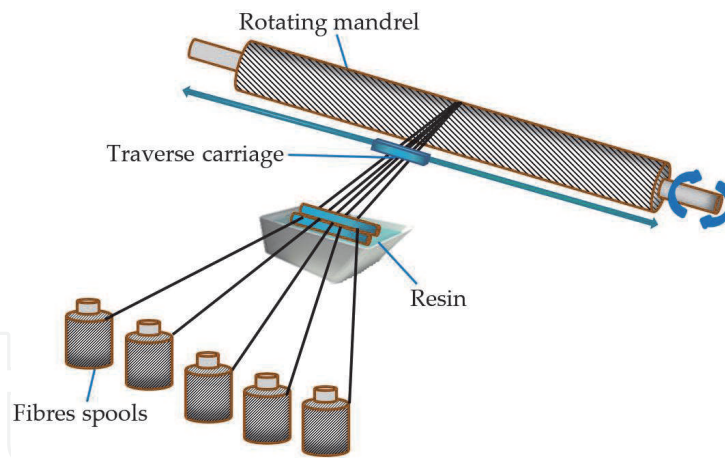
Figure 9. The schematic of the filament winding process.
