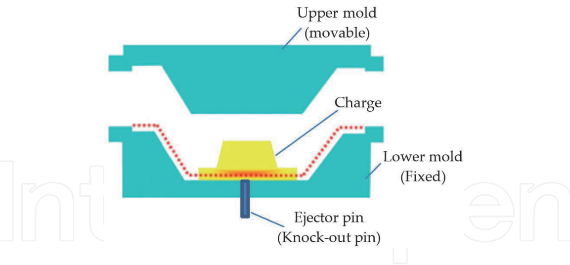
Figure 7. The schematic of compression moulding process.
