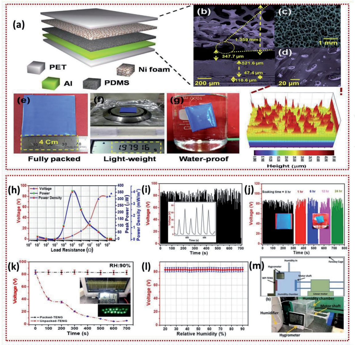
Figure 10. (a) Schematic and layers of waterproof TENG device. (b–d) FESEM image showing the cross-section of WP-TENG device with both the layers, morphology of nickel foam and roughness PDMS. (e) Fully packed device. (f) Lightweight device weight. (g) Waterproof capability. (h) Load resistance vs. power density analysis. (i) Rectified voltage. (j) Water-resistant analysis with different time duration (k and l) humidity with output analysis. (m) Homemade humidity chamber for the analysis [34].
