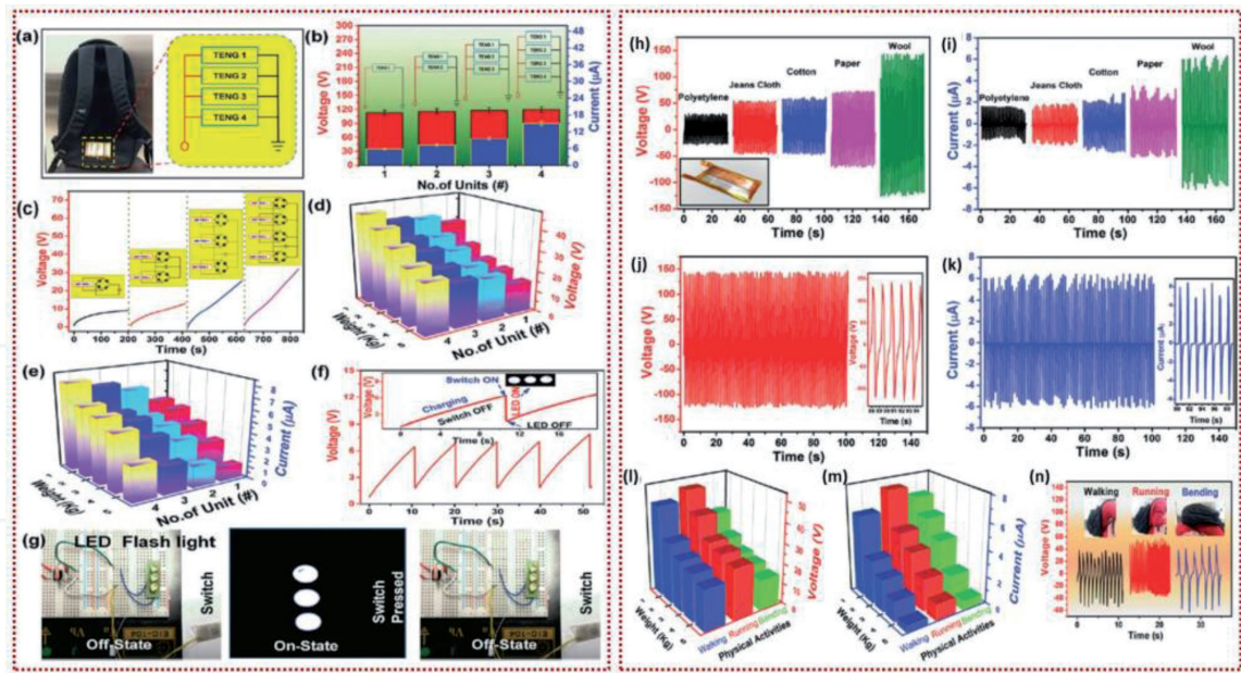
Figure 7. (a–e) Electrical response of SBP-TENG device showing its electrical response under parallel connections with four units. (f) Cyclic stability study by charging and discharging a 1 \mu F capacitor. (g) Emergency LED flash using a switch and a capacitor. (h and i) Electrical response of SBP-TENG with various contact materials and the maximum response obtained with wool. (j and k) Voltage and current responses of SBP-TENG with wool. (l–n) The electrical response of SBP-TENG under biomechanical motions such as walking, running, and bending [39].
