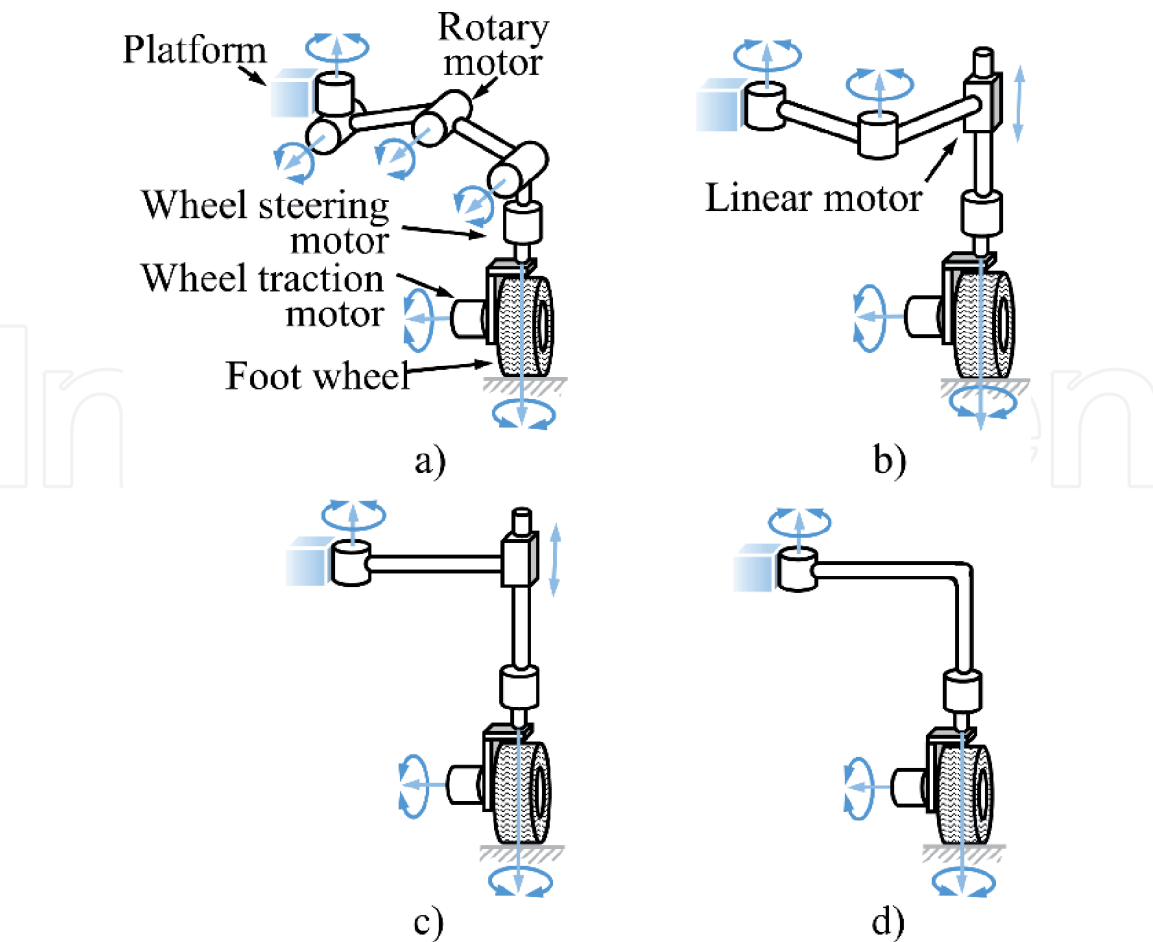
Figure 5. Wheel-legged structures. (a) 4-DOF articulated leg; (b) 3-DOF SCARA leg; (c) 2-DOF SCARA leg; (d) 1-DOF leg.
