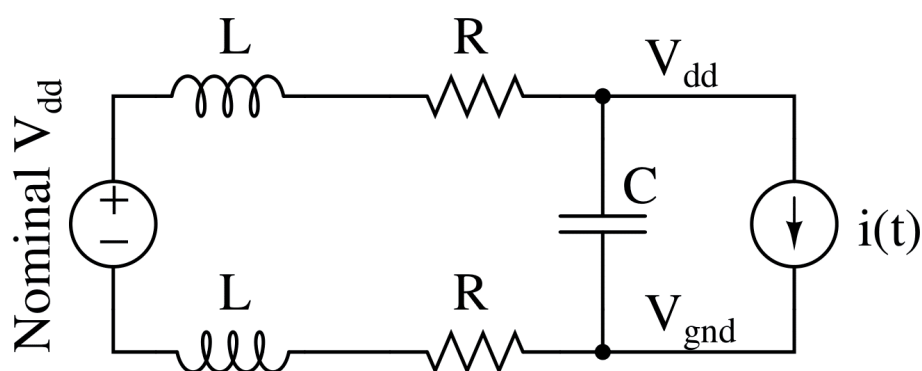
Figure 2. Simplified circuital scheme of power distribution system.
