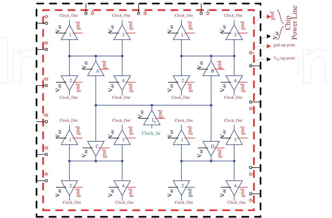
Figure 3. H-type balanced clock tree network as a part of CDN.
