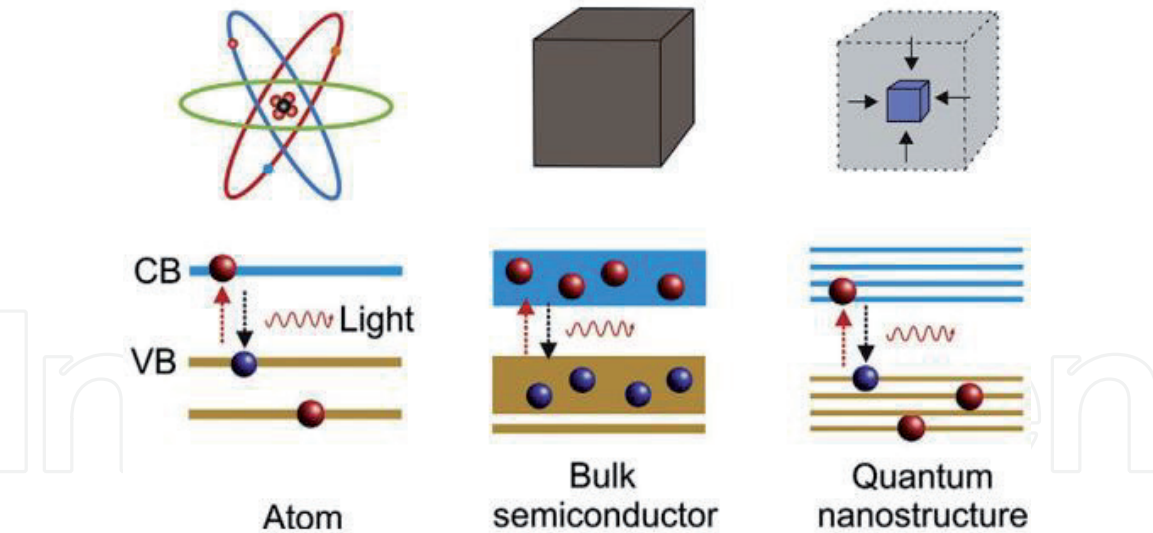
Figure 1. Schematic diagram showing energy band structures in atom, bulk semiconductor, and quantum nanostructure.
