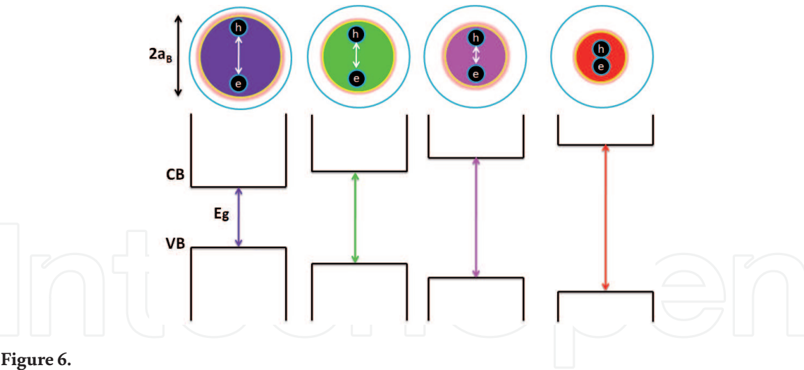
Figure 6. Quantum confinement in semiconductor crystal.
