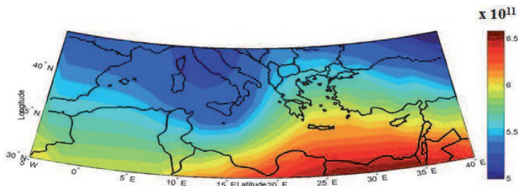
Figure 14. Map of the ionospheric electron density in \text{el/m}^3 at the fixed height of 201 km obtained by the IRI-SIRMUP-P procedure for a given epoch.
