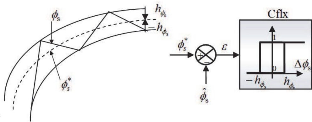
Figure 3. Two-level hysteresis comparator for stator flux control.
