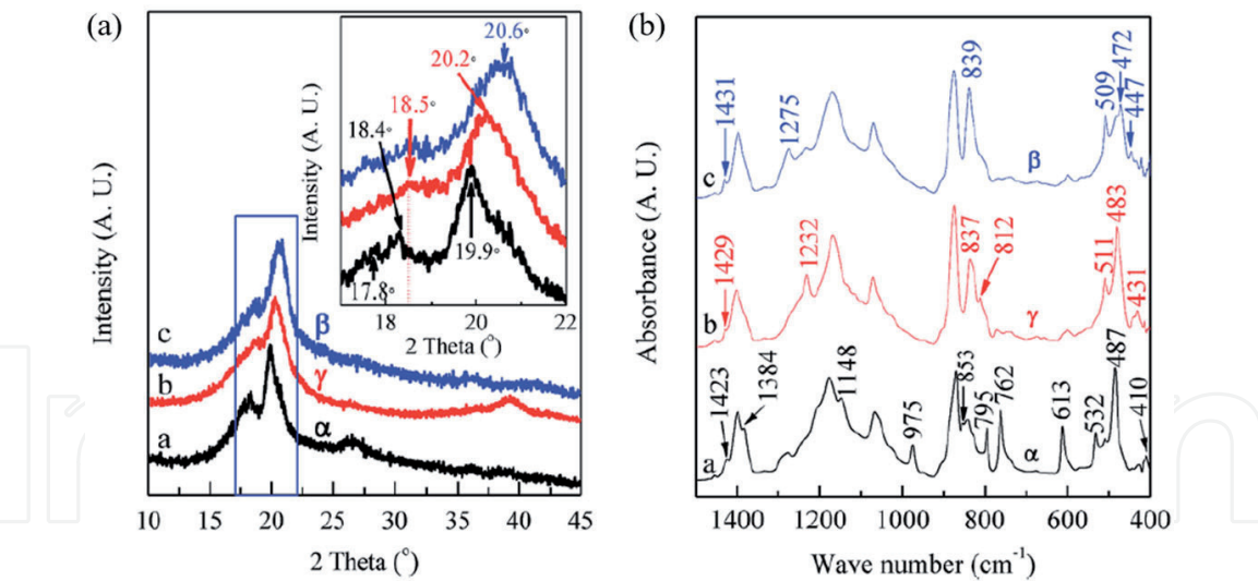
Figure 2. XRD patterns (A) and FTIR spectra (B) of PVDF membranes [33].
