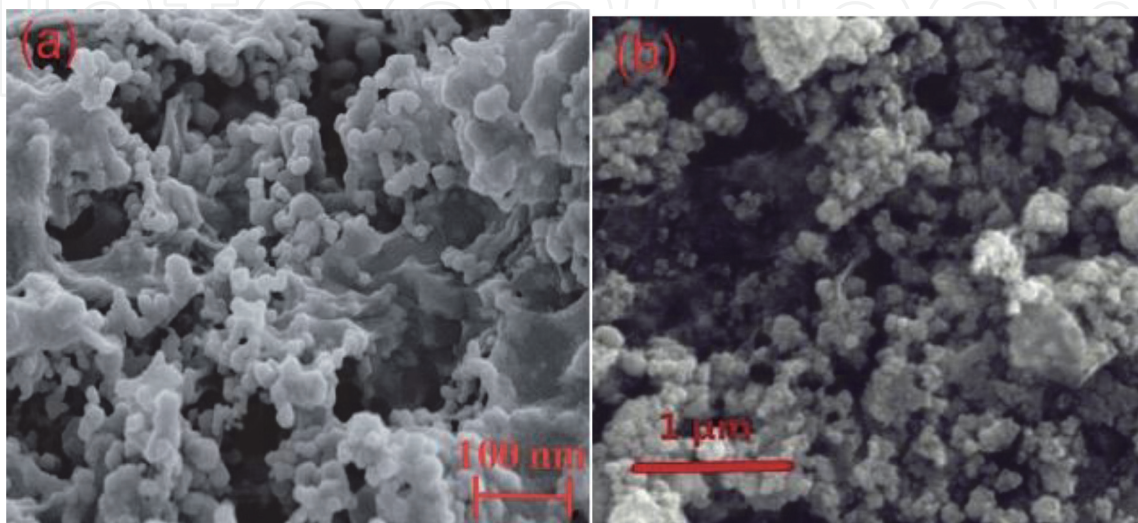
Figure 1. SEM image of hydrothermally grown \text{SnO}_2 nanoparticles and rGO composites reported by (a) Zhang et al. [33] and (b) Peng et al. [41].
