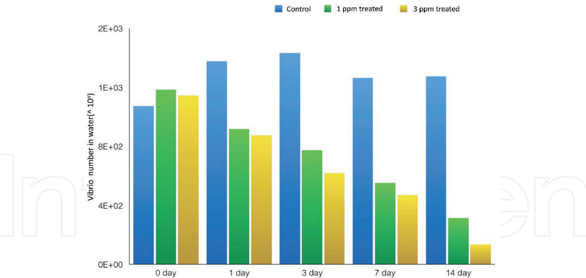
Figure 1. Effectiveness of photosynthetic bacteria applied in white shrimp culture. Change in the total amount of Vibrio in the culture pond within 14 days of continuous use of photosynthetic bacteria in the white shrimp culture process. The results showed that in the experimental group with more than 1 ppm of photosynthetic bacteria added continuously, the total amount of Vibrio was significantly reduced, which proved that the use of photosynthetic bacteria can effectively reduce the number of Vibrio in water.
