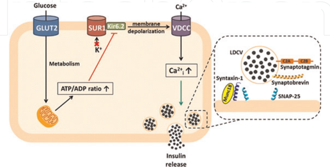
Figure 4. Glucose-stimulated insulin release from a pancreatic \beta -cell.
