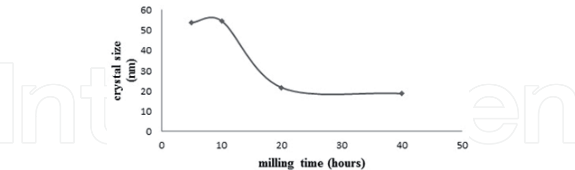
Figure 11. Effect of milling time on crystal size.
