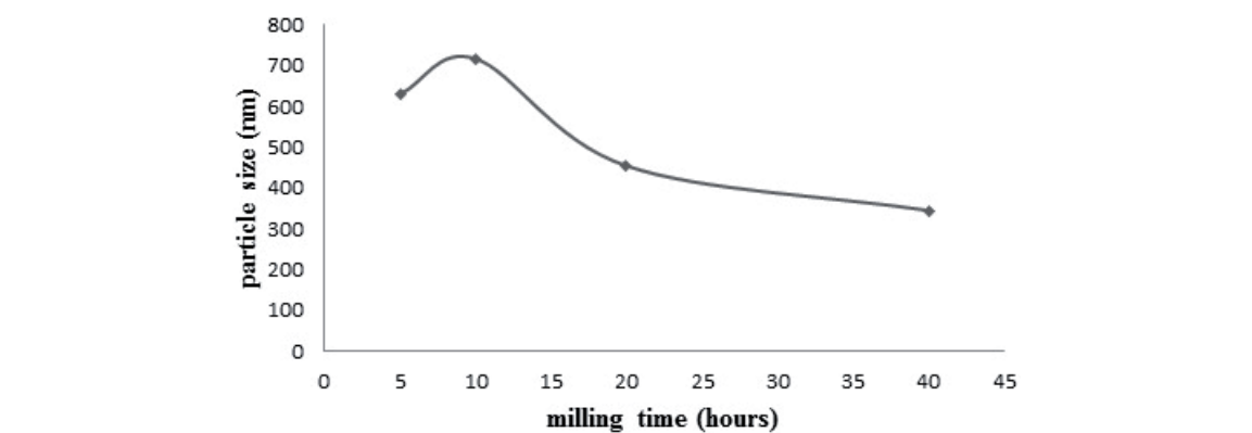
Figure 13. Effect of milling time on grain size.
