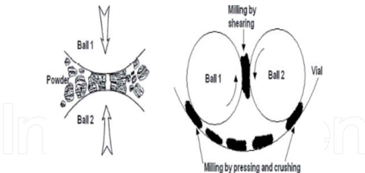
Figure 5. Concept of powder destruction at ball mill [29].
