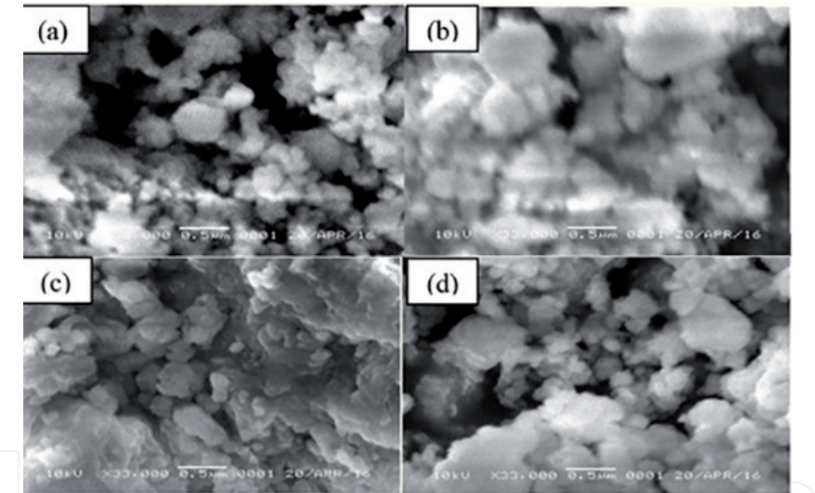
Figure 12. Differences in the form of morphology in each milling time variation with a magnification of 33,000 \times . (a) 5 h, (b) 10 h, (c) 20 h, (d) 40 h.
