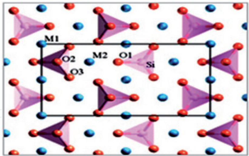
Figure 2. Crystal structure of olivine [12].
