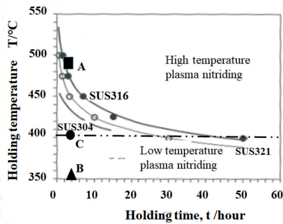
Figure 18. Relationship of the holding temperature to the holding time in the plasma nitriding.
