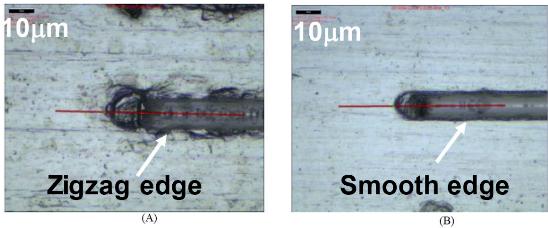
Figure 4. Picture after microcutting by diamond tool. (A) Left: groove condition on normal grain stainless steel. The average grain size is 9.8\text{ }\mu\text{m} and (B) right: Groove condition on FGSS by reverse phase transformation. The average grain size is 1.52\text{ }\mu\text{m} . FGSS can get smooth edge when cutting in microscale.
