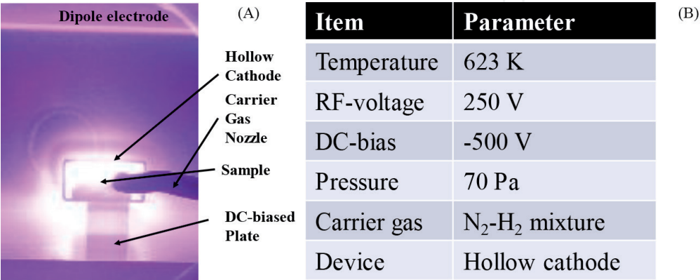
Figure 19. High density plasma nitriding system with use of the hollow cathode for low temperature plasma nitriding of FGSS316. (A) Schematic view of nitriding system, and (B) plasma nitriding conditions in the following experiments.
