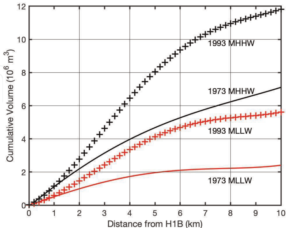
Figure 13. Cumulative volume of water in ES at MLLW and MHHW from Smith [10] and as re-evaluated in 1993 from more recent aerial photographs. The volume between MLLW and MHHW is defined as the tidal prism, and estimated to be 4.7 \times 10^6 \text{ m}^3 in 1973 and 6.2 \times 10^6 \text{ m}^3 in 1993.
