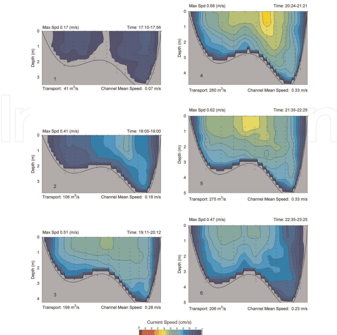
Figure 11. ADP vertical sections of along-channel currents 250 m east of H1B show vertical and horizontal shear. The north shore is on the right. These data were obtained through a flood tide cycle on 2 January 2003. The integrated transport was 4.9 \times 10^6 \text{ m}^3 .
