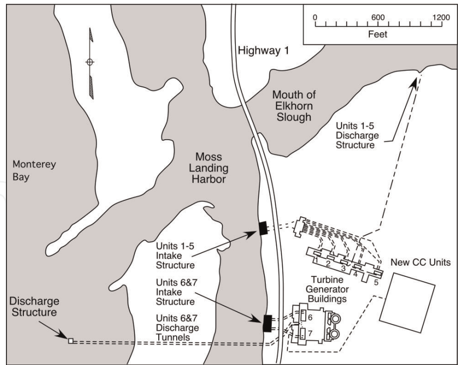
Figure 2. Moss Landing Harbor, adapted from Duke Energy Moss Landing [10].
