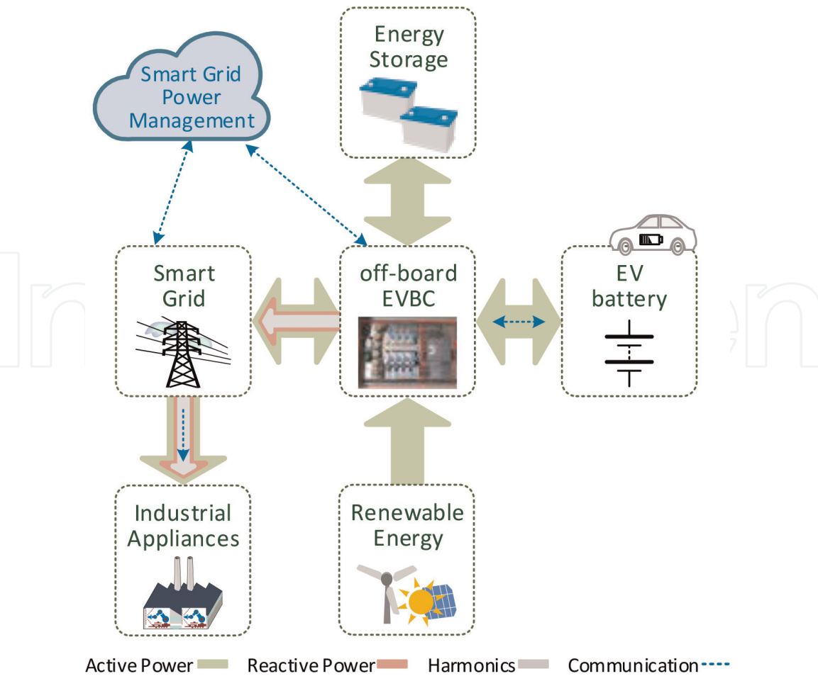
Figure 27. An off-board EVBC with an EV plugged-in into the electrical power grid: unified operation with RES, ESS, and as a power quality compensator.
