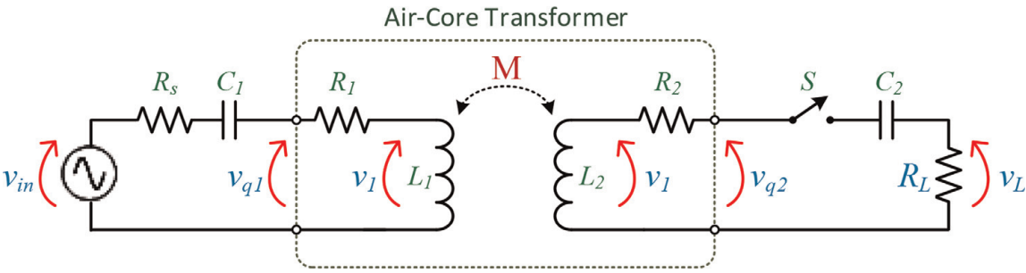
Figure 7. Simplified circuit analysis for the SS-compensated WPT.
