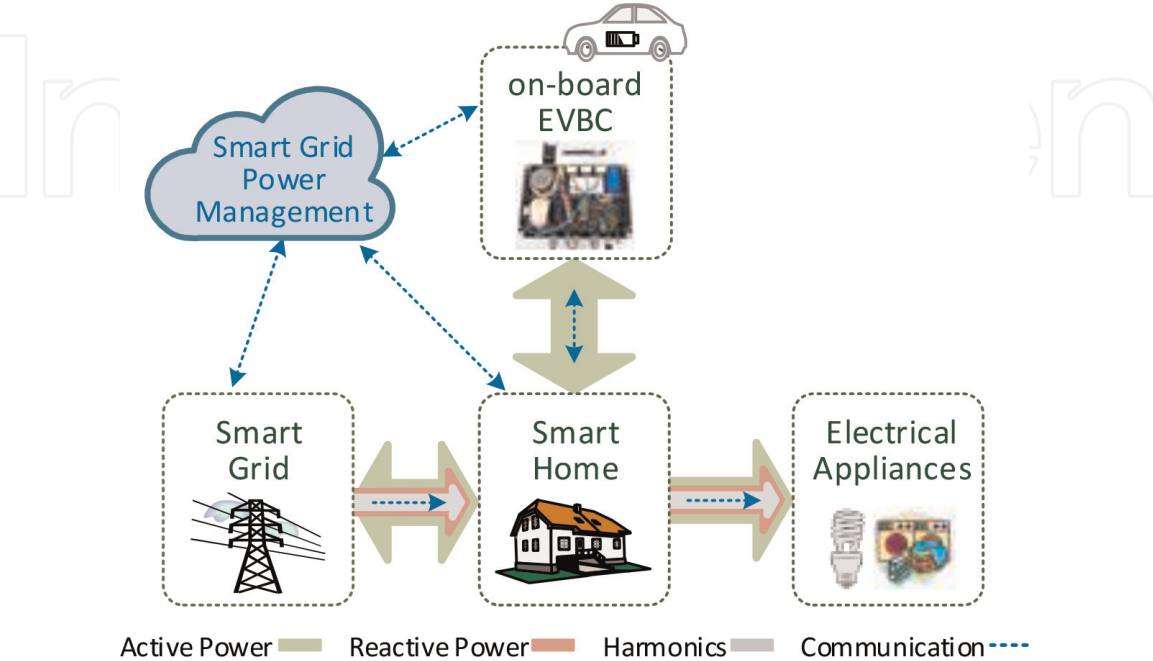
Figure 20. On-board EVBC: V2G operation mode.
