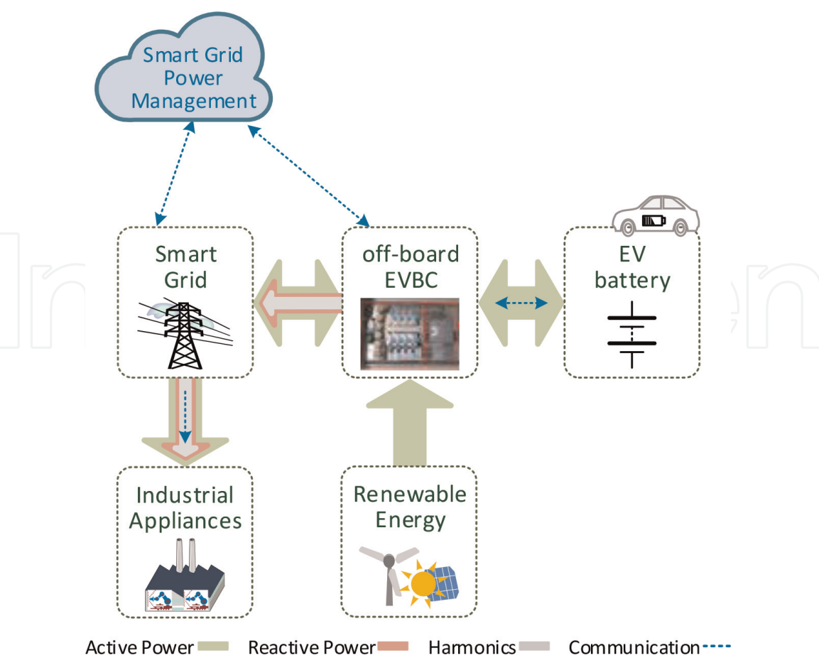
Figure 26. An off-board EVBC with an EV plugged-in into the electrical power grid: unified operation with RES and as a power quality compensator.
