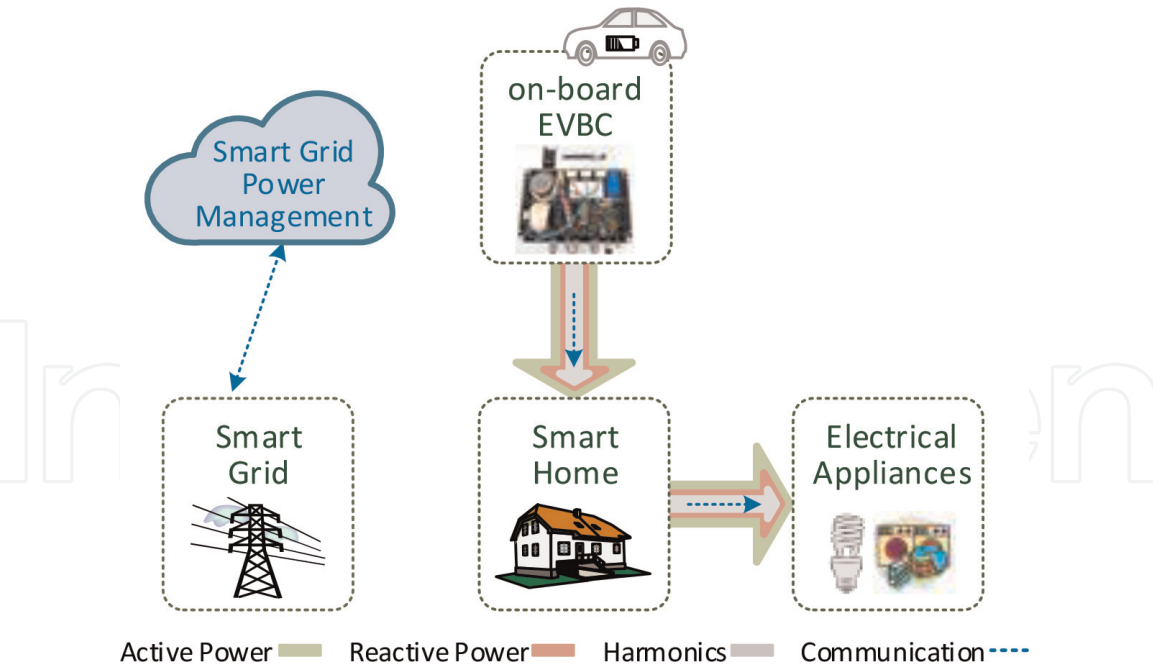
Figure 22. On-board EVBC: V2H operation mode (as an off-line uninterruptible power supply).
