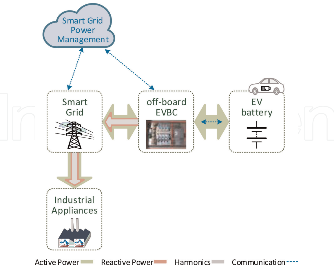
Figure 25. An off-board EVBC with an EV plugged-in into the electrical power grid: operation as a power quality compensator.
