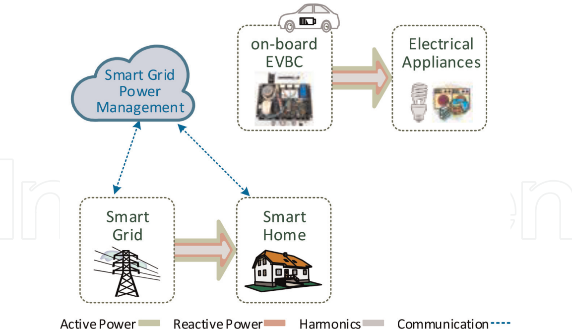
Figure 21. On-board EVBC: V2L operation mode (as a voltage source).
