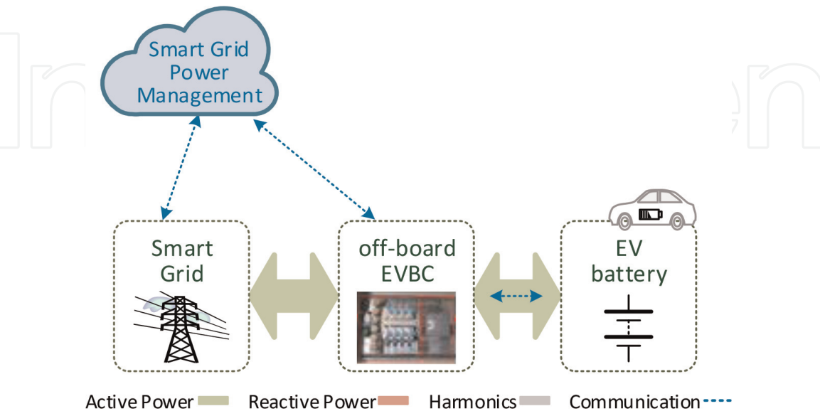
Figure 24. An off-board EVBC with an EV plugged-in into the electrical power grid: G2V/V2G modes.
