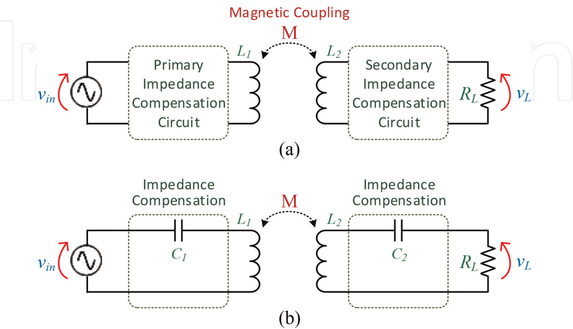
Figure 6. Basic WPT configuration: (a) exemplified with the series-series (SS) impedance; (b) impedance compensation.
