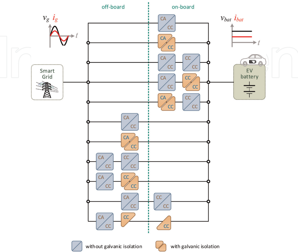
Figure 2. Possible structures that can be implemented in EVBC, highlighting on-board and off-board concepts, as well as power stages encompassing a galvanic isolation.
