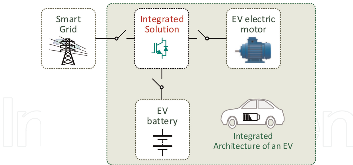
Figure 17. Integrated architecture of an EV used for two purposes: On-board EVBC and EV motor driver.
