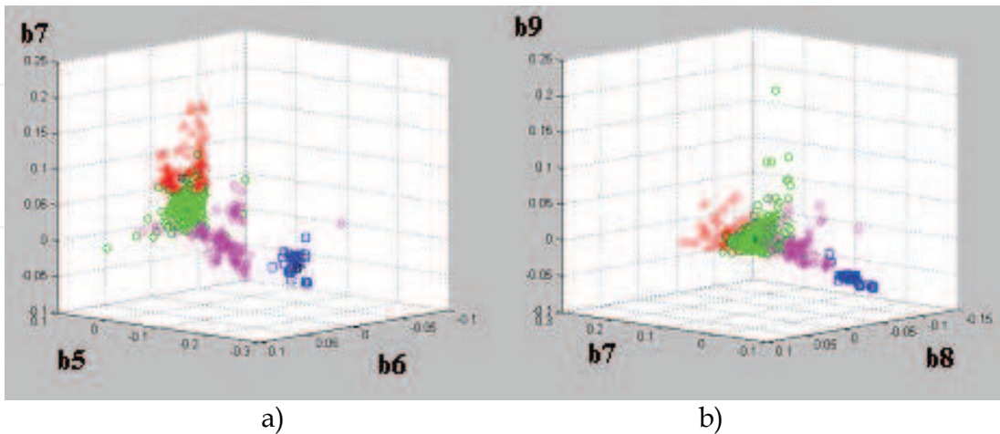
Fig. 7. The cluster identification using the sensors values b5, b7, b7 (a) and b7, b8, b9 (b)
