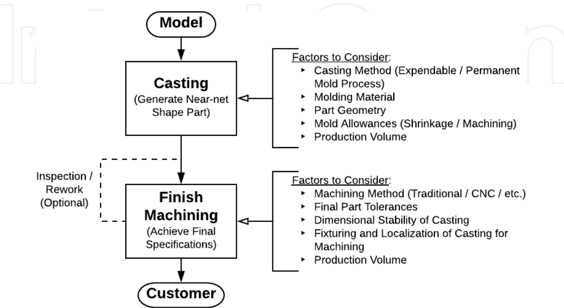
Figure 1. Process flow of casting-subtractive category of HMP.
