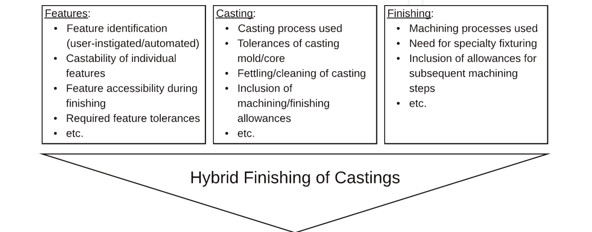
Figure 6. Considerations for casting-subtractive HMP process planning.
