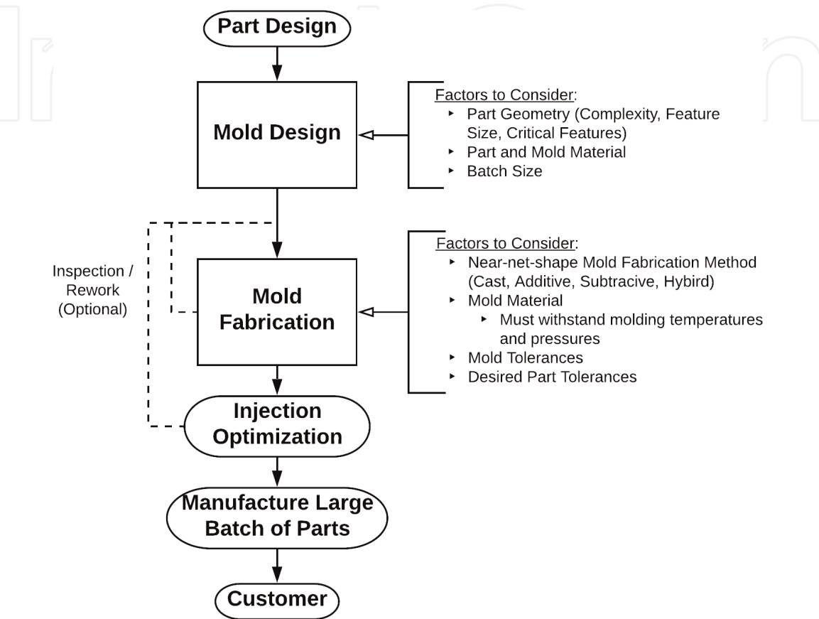
Figure 2. Process flow for creating injection molded parts for large batch scenarios.
