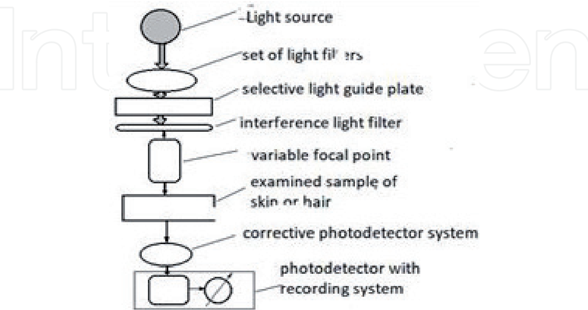
Figure 1. The block diagram of the installation for the investigation of spectral optical characteristics of the cover of animals.
