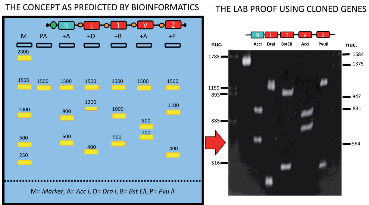
Figure 4. Diagnostic test for the hGH locus. Bioinformatics prediction and confirmation in the laboratory of the PCR + restriction enzymes test to differentiate each of the five genes constituents of the hGH locus. The gene-specific digestion patterns predicted in silico when amplifying all genes by a simple consensus primers PCR and then subjecting the pentagenic amplicon to “diagnostic” restriction enzymes were confirmed using cloned versions of all the gene members of this gene family.
