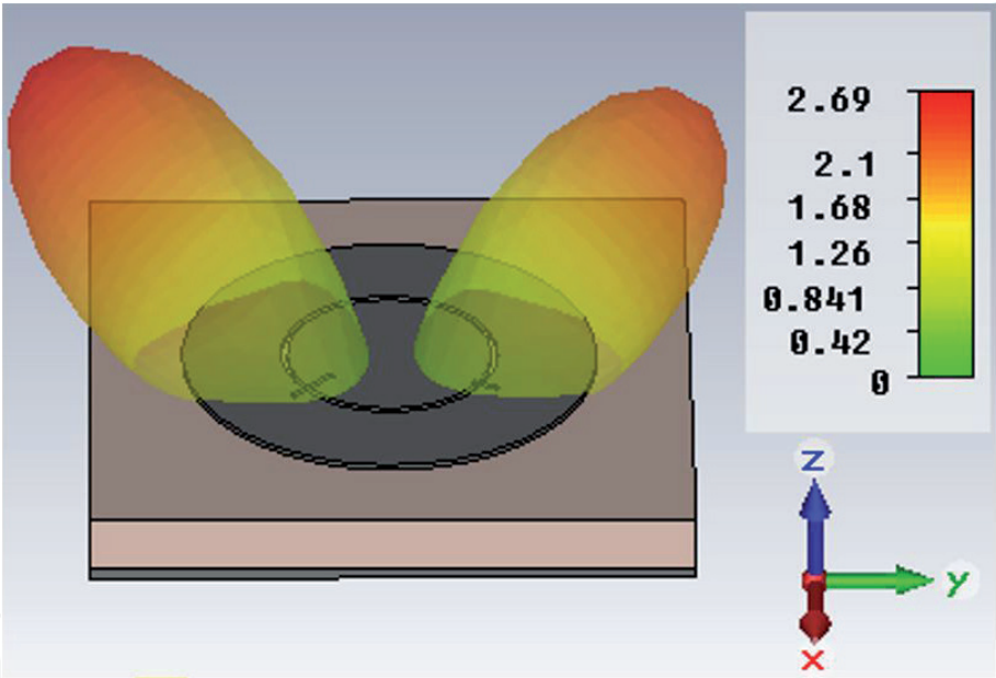
Figure 14. 3D radiation pattern in the ON-ON state.
