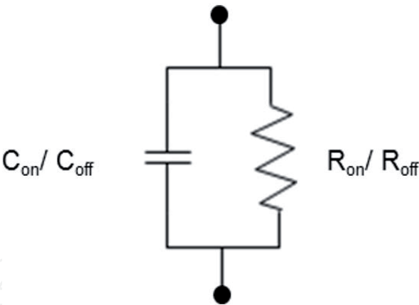
Figure 6. Simplified electrical model of the NMOS transistor switch in ON and OFF states.
