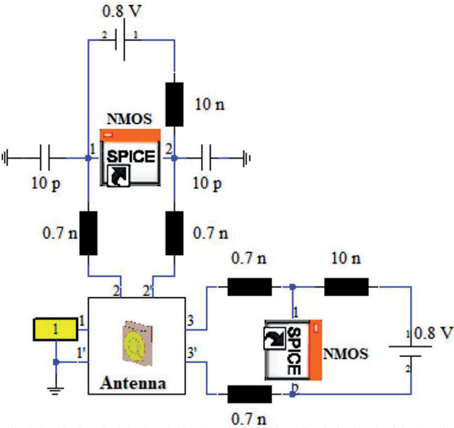
Figure 7. A hybrid EM-circuit co-simulation of the antenna.
