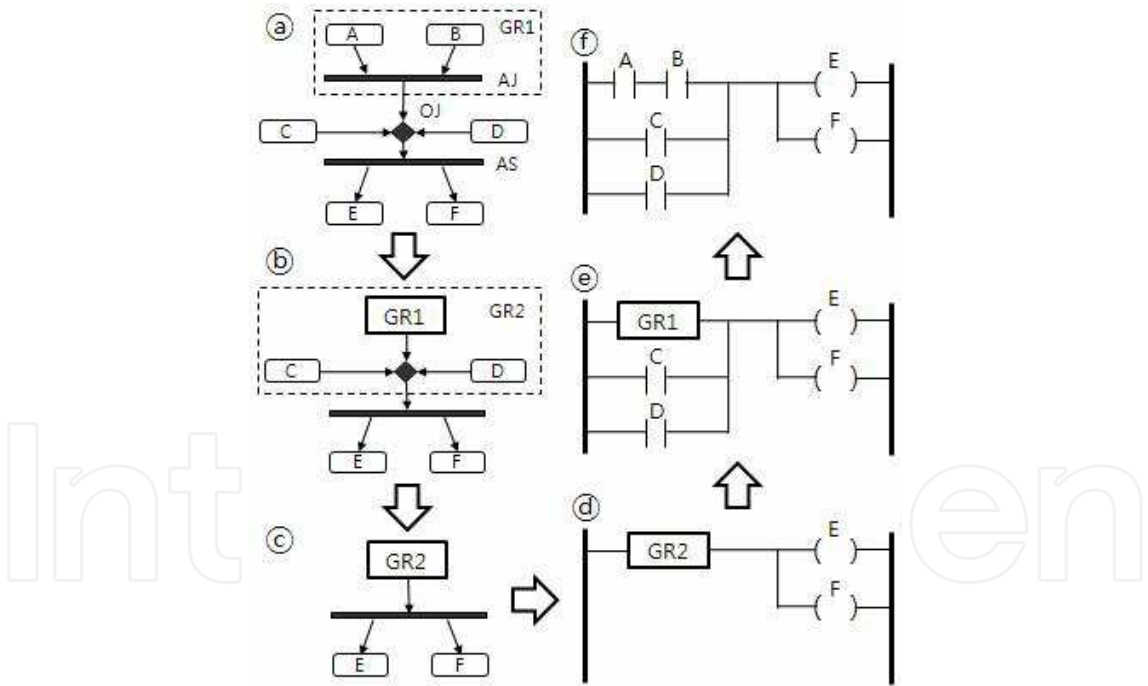
Fig. 12. Transformation procedure of join-precedent type 5-1
