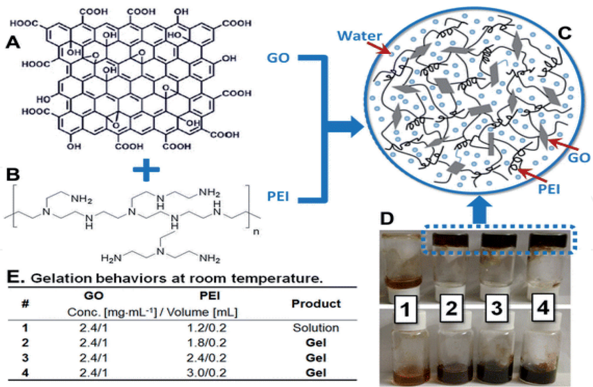
Figure 1. Schematic representation of the formulation of GO/PEI hydrogel. (A) GO, (B) PEI, (C) GO/PEI hydrogels, and (D) and (E) are the gelation pictures [35].
