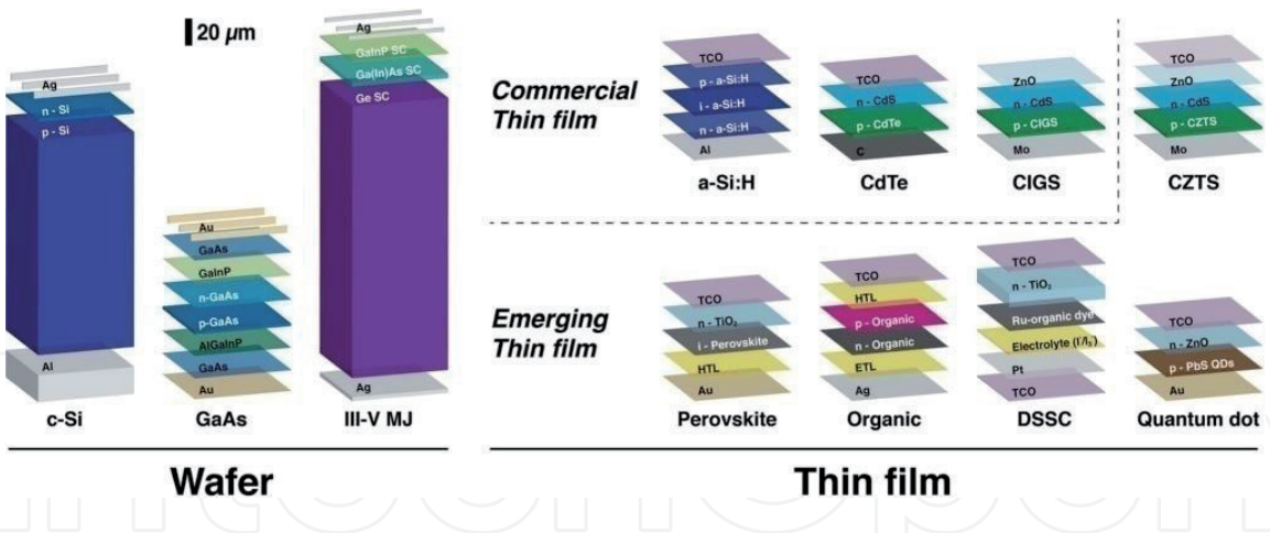
Figure 1. Typical PV device structures, divided into thin film and wafer-based technologies. Primary absorber layers are labeled in white color, and thicknesses are shown to scale (obtained under copyright of Royal Society of Chemistry [2]).
