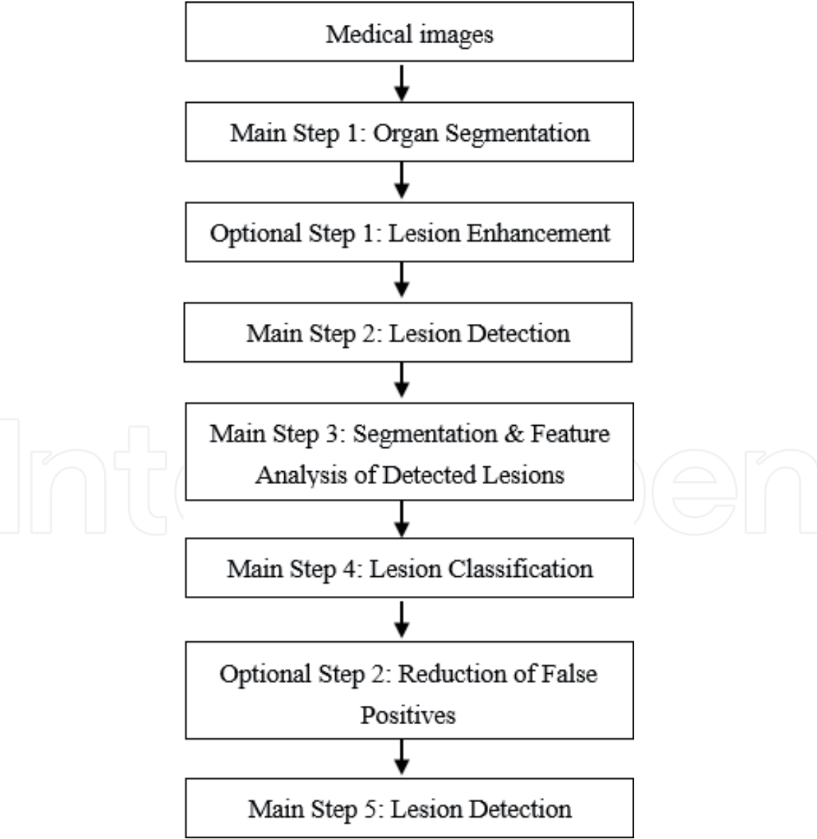
Figure 1. Flowchart of computer-aided detection [11].
