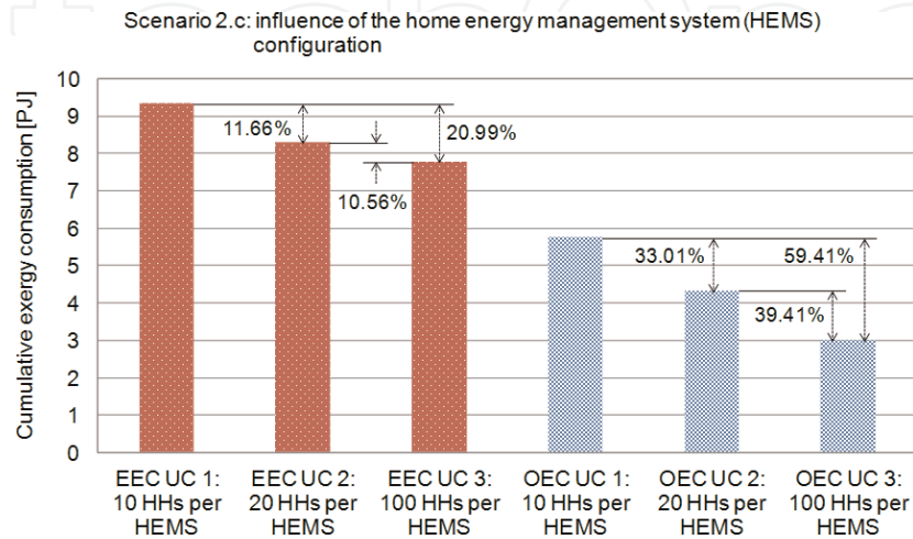
Figure 13. Distribution of the cumulative embodied exergy consumption (EEC) and operational exergy consumption (OEC) of Scenario 2.c for the three defined use cases (UCs) with different numbers of households (HHs) per home energy management system (HEMS), after an operational duration of 20 years.
