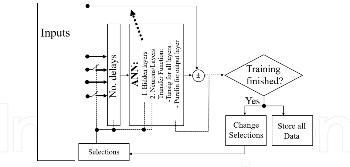
Figure 9. The architecture of the neural network modeling.
