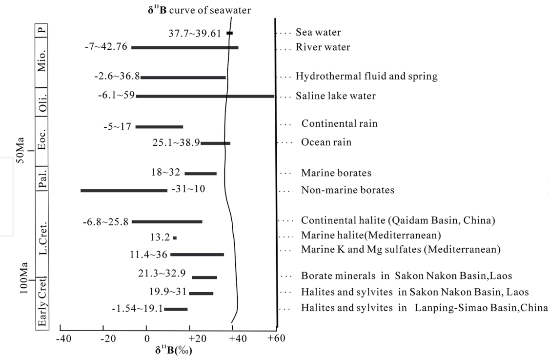
Figure 16. \delta^{11}\text{B} values from published papers. Marine and nonmarine borates after Swihart et al. [91], Xiao et al. [90], and Palmer and Helvacı [85]. Seawater after Vengosh et al. [86] and Foster et al. [89]. River water after Vengosh et al. [7]; Rose et al. [92]; and Lemarchand et al. [93]. Halite after from Vengosh et al. [86]; Liu et al. [94]; and Kloppmann et al. [95]. Borate minerals in SNB after Zhang et al. [96]. Halite and sylvite in SNB after Tan et al. [66]). Halite and sylvite in LSB after Zhang et al. [97]. Curve of seawater after Lemarchand et al. [98].
