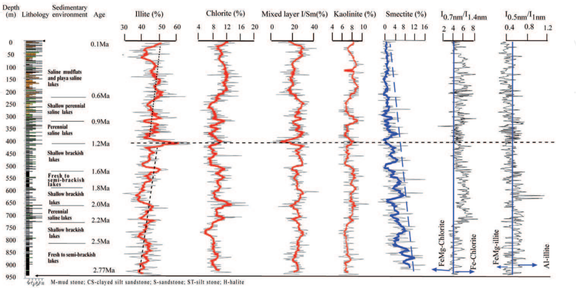
Figure 3. Variations in the amount of illite, chlorite, kaolinite, smectite, and illite/smectite (I/Sm) and in the chemistry of illite ( I_{5\text{\AA}}/I_{10\text{\AA}} ratios) and chlorite ( I_{7\text{\AA}}/I_{14\text{\AA}} ratios). Colored lines represent a five-point running average. Sedimentary environments are from Wang et al. [10]; ages are from Zhang et al. [9].
