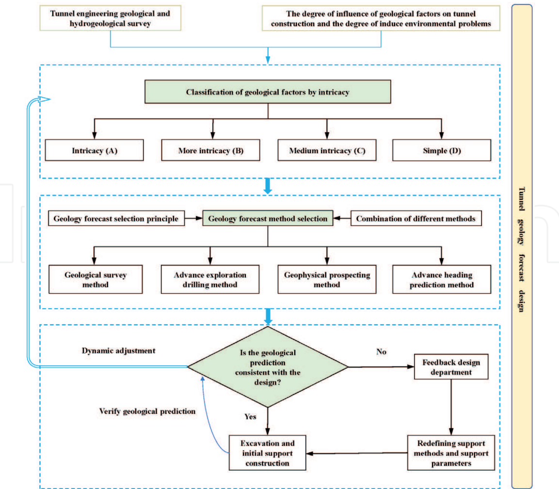
Figure 2. Flow chart of tunnel geology forecast design.
