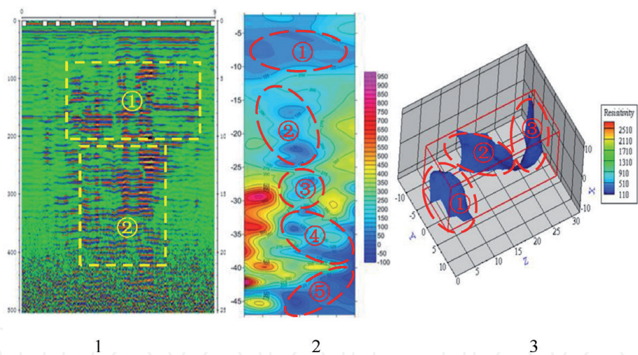
Figure 4. Comparison of detection results. (1) Geological radar detection results; (2) transient electromagnetic detection results; (3) excited excitation detection result (hole body range extraction map).
