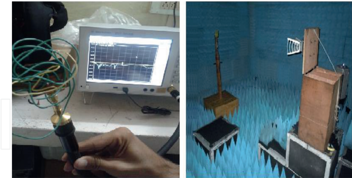
Figure 11. Images of measurement setup for proposed antenna.
