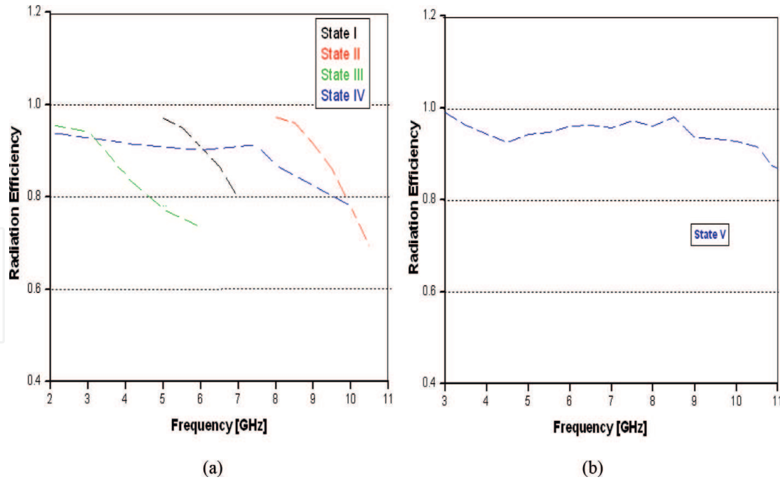
Figure 16. Simulated radiation efficiency of the proposed antenna for different switching states: (a) single-band and dual-band modes and (b) UWB.
