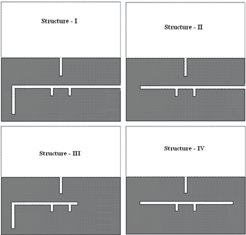
Figure 5. Filter structures placed on the ground plane.
