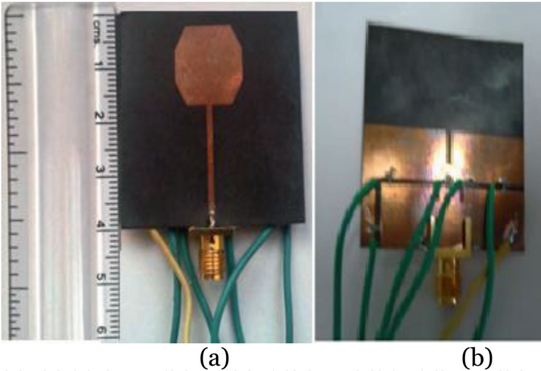
Figure 10. Images of the fabricated antenna: (a) top view and (b) bottom view.
