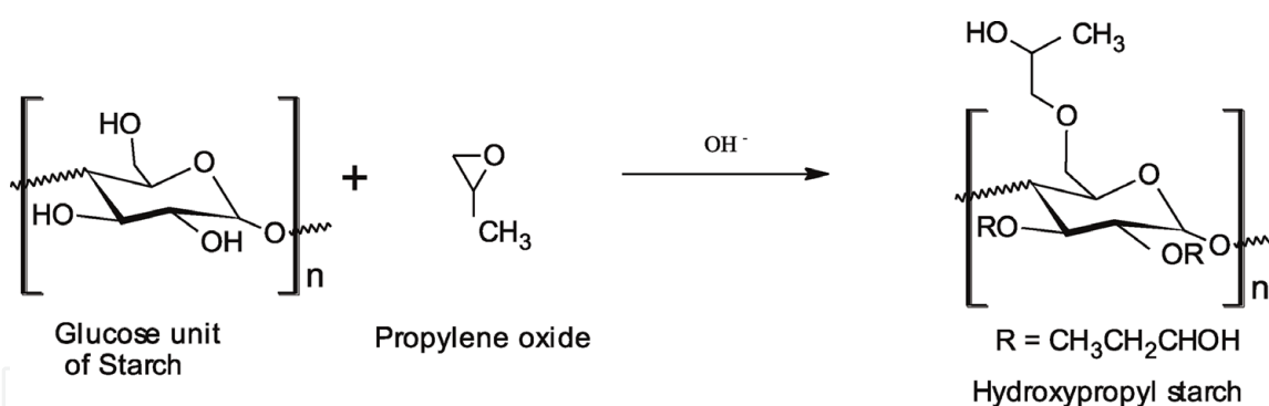
Figure 14. Etherification of starch with propylene oxide.
