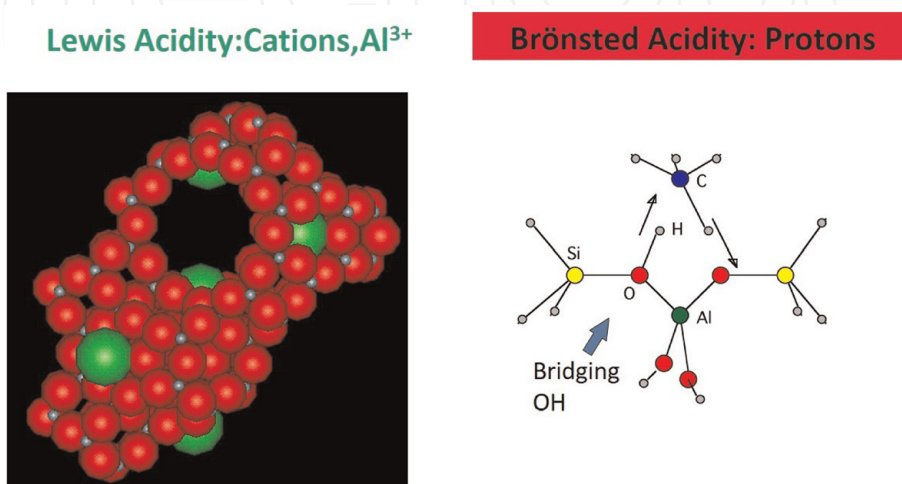
Figure 3. Scheme of Lewis and Brönsted acidity of single bonds. The substitution of tetravalent Si atoms in the lattice with the trivalent Al atoms generates local negative charges, which are then compensated by extra-framework cations. The charge compensation by protons results in strong Brönsted acid sites.
