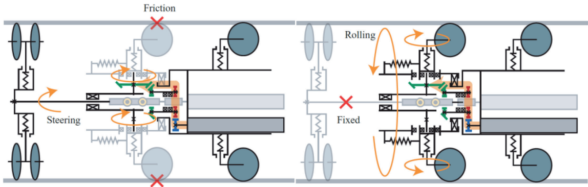
Figure 4. Steering mode and rolling mode using a miter-gearred differential mechanism.
