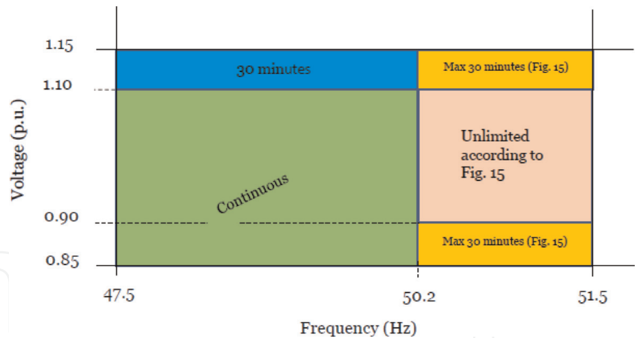
Figure 14. Voltage, frequency, and time ranges of solar plant operation.
