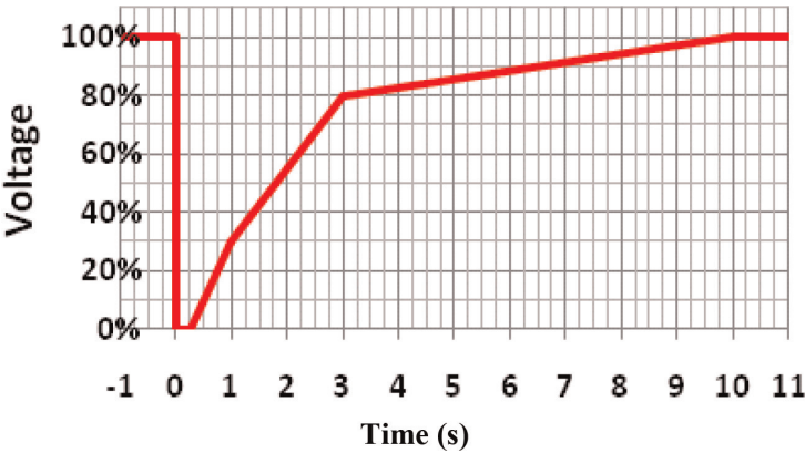
Figure 18. Low voltage ride-through curve of solar plants.
