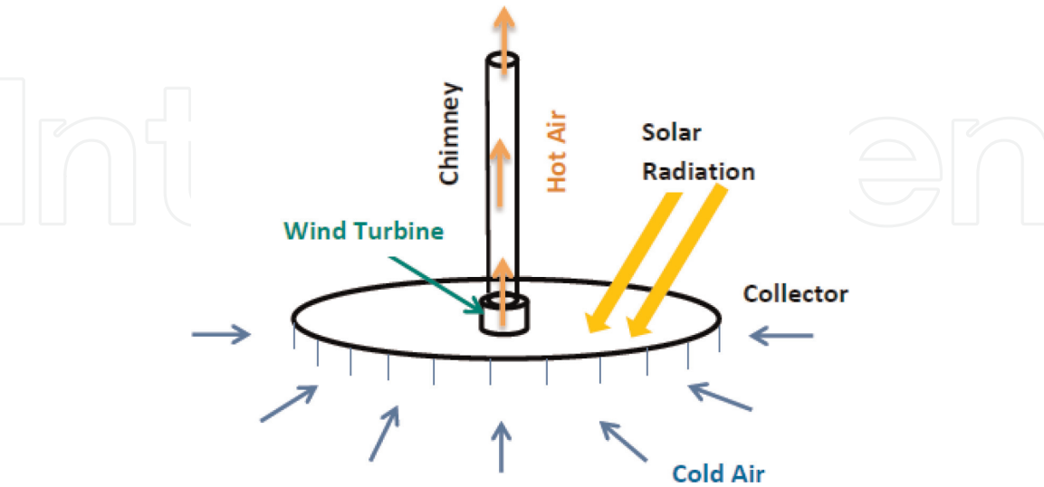
Figure 8. Concept of solar chimney.
