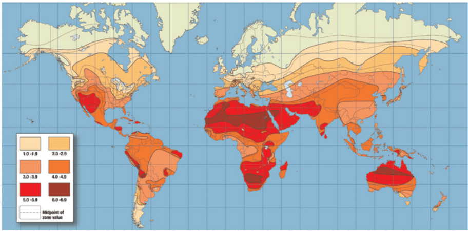
Figure 1. Annual solar insolation worldwide [12].
