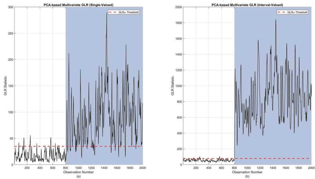
Figure 12. PCA-based multivariate GLR charts (IDV 3).
