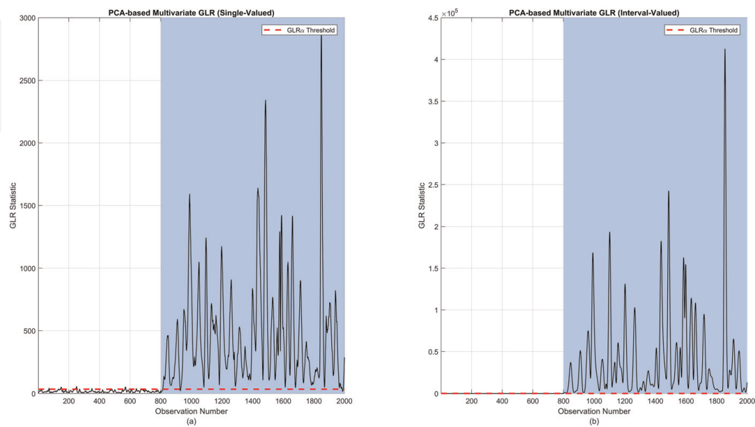
Figure 13. PCA-based multivariate GLR charts (IDV 11).
